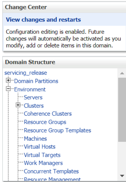
Figure 7-1 Domain Structure
