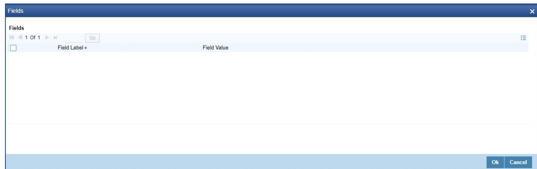
Figure 2-14 UDF Button
