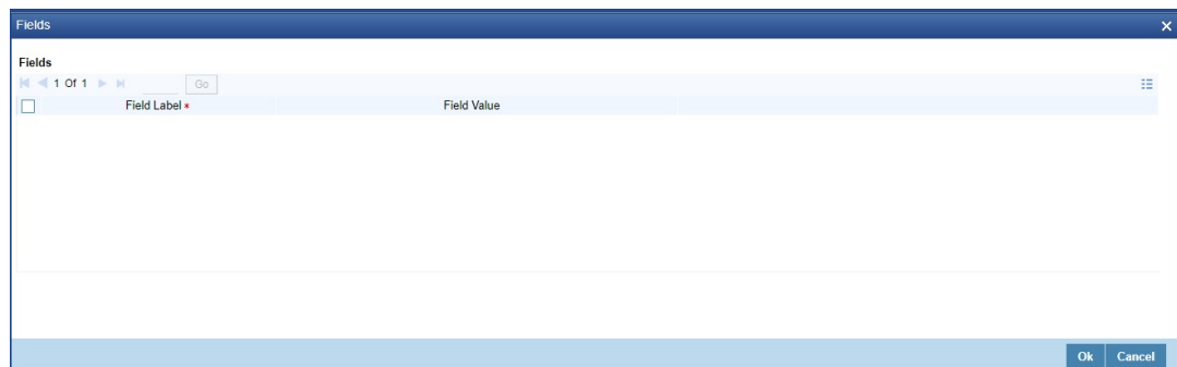
Figure 3-61 UDF Button
