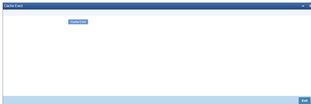
Figure 3-64 Cache Evict
