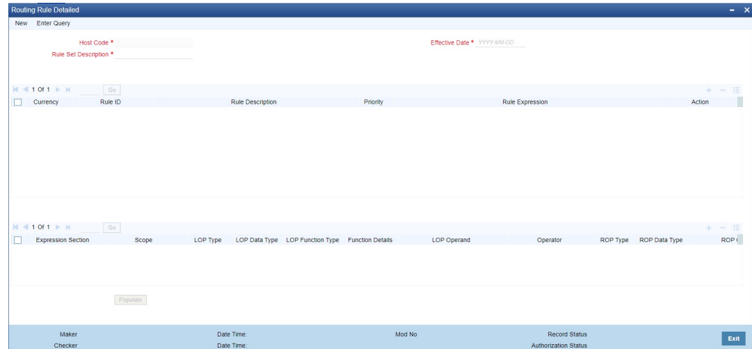
Figure 2-295 Routing Rule
