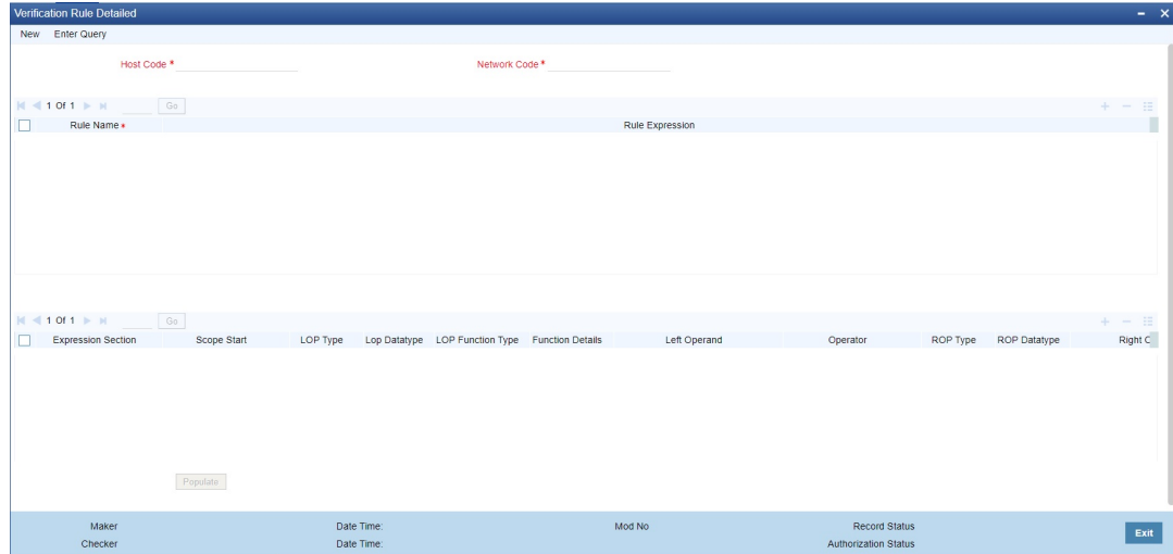
Figure 2-224 Verification Rule
