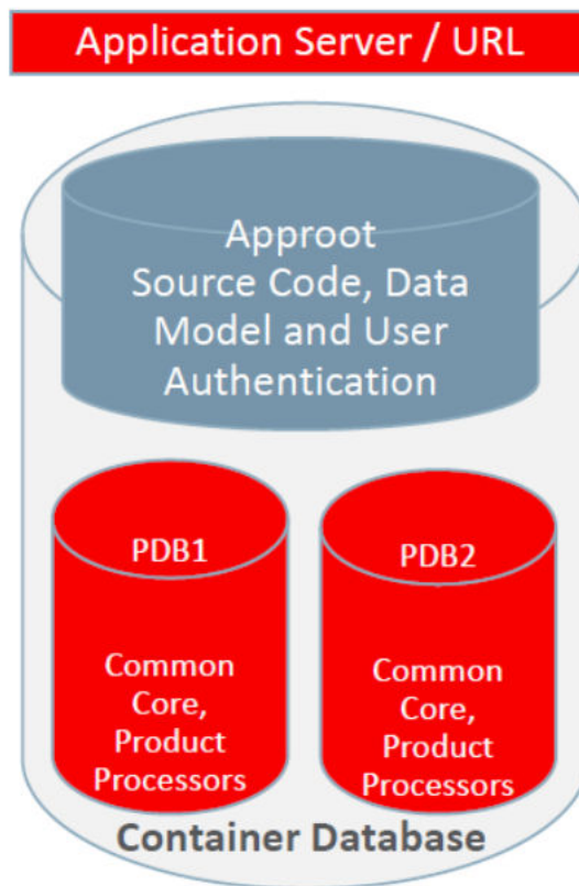
Figure 3-2 Shared Application and User Authentication
