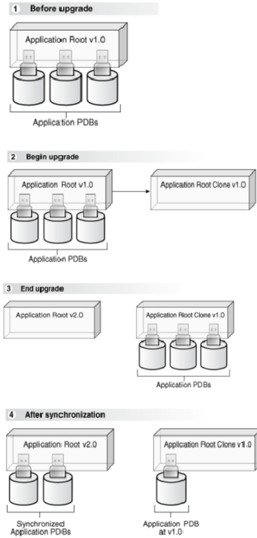
Figure 2-2 Application Upgrade Process
