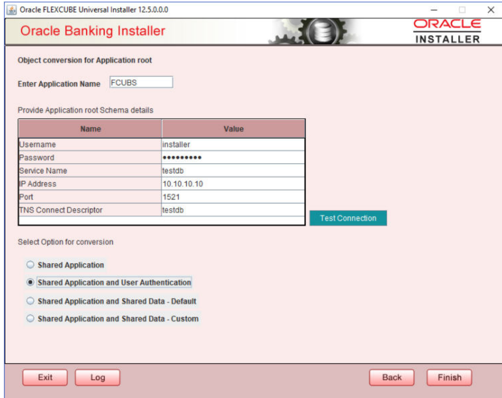
Figure 5-9 Object Conversion for Application Root
