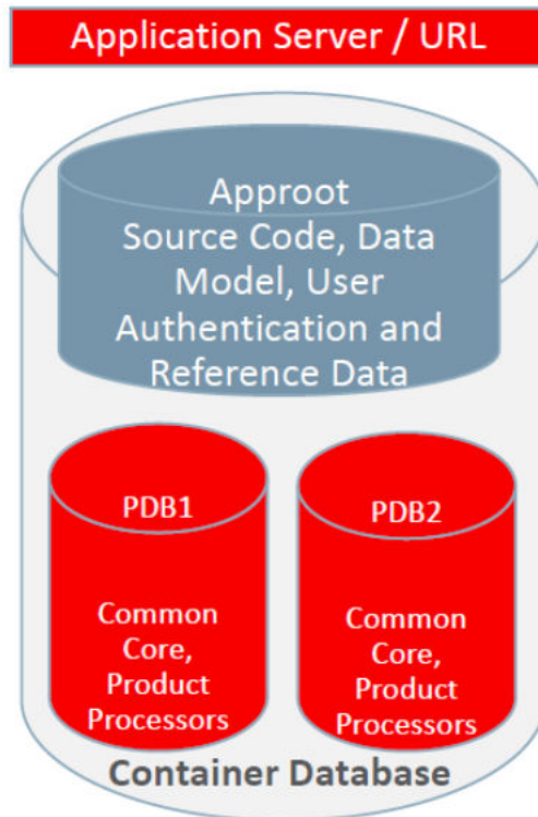
Figure 3-3 Shared Application with Shared Data - Default
