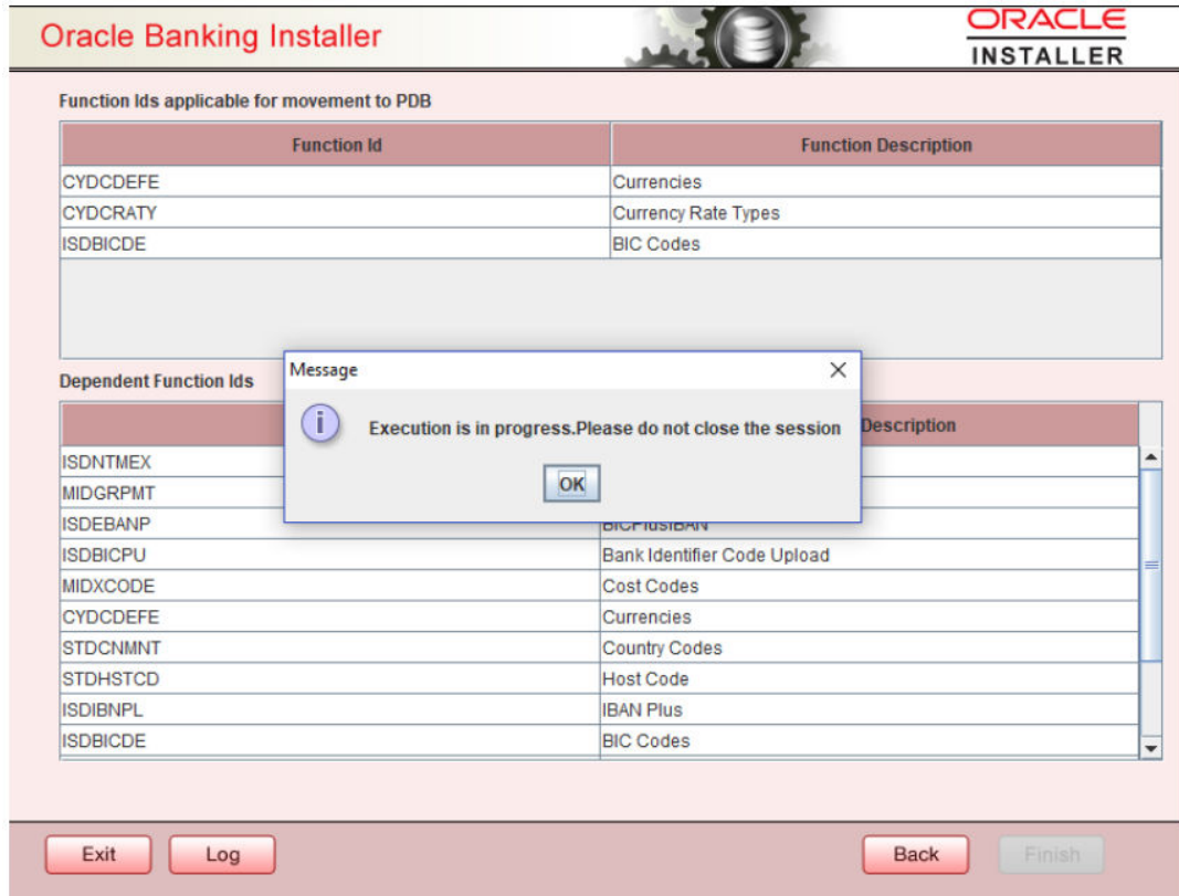
Figure 5-23 Function Ids applicable for movement to PDB
