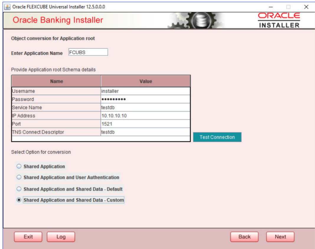
Figure 5-19 Object Conversion for Application Root
