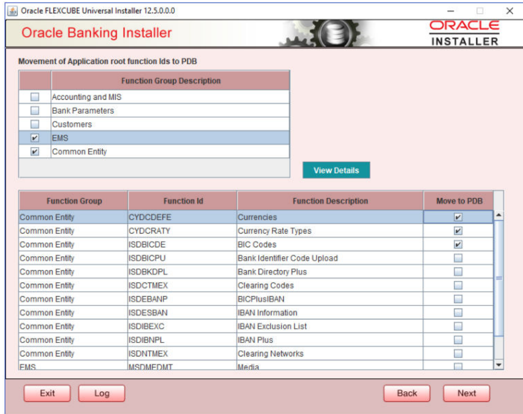
Figure 5-21 Movement of Application root function Ids to PDB
