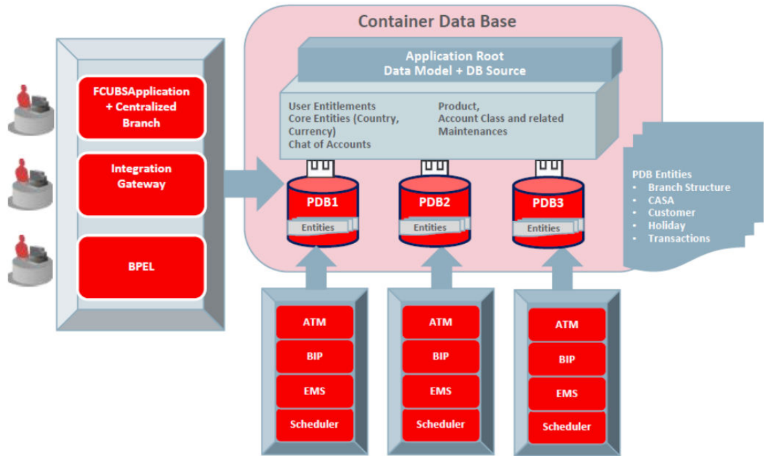
Figure 3-4 Component Deployment Architecture
