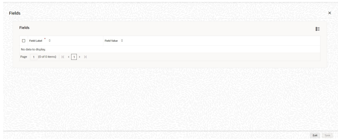
Figure 1-17 UDF Button
