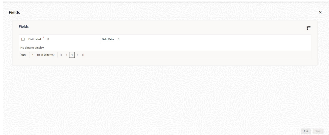
Figure 1-26 UDF Button
