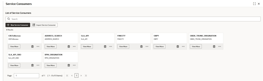
Figure 1-6 Service Consumers
