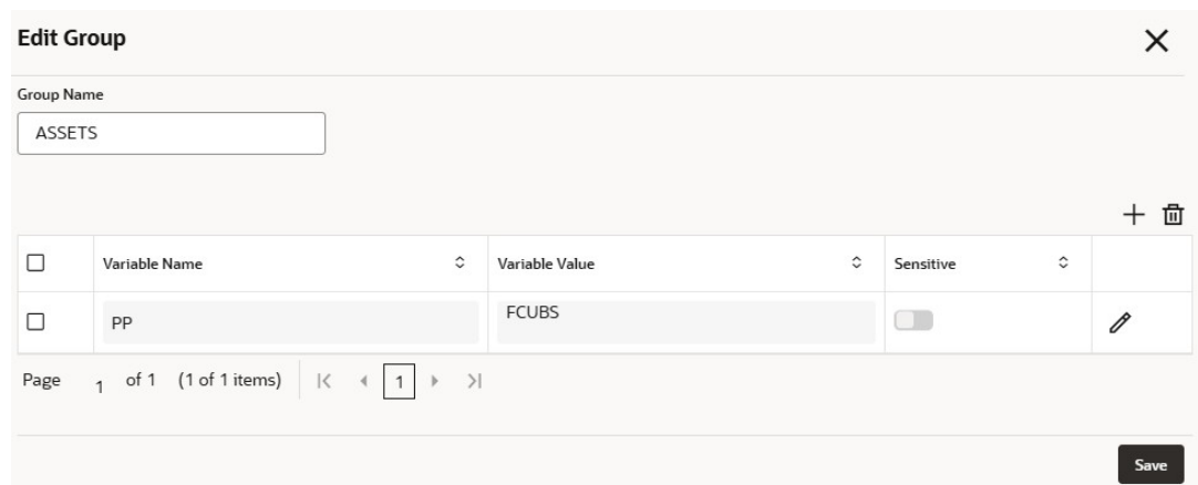
Figure 1-15 Edit Group
