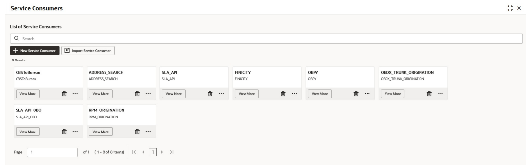
Figure 1-13 Service Consumers
