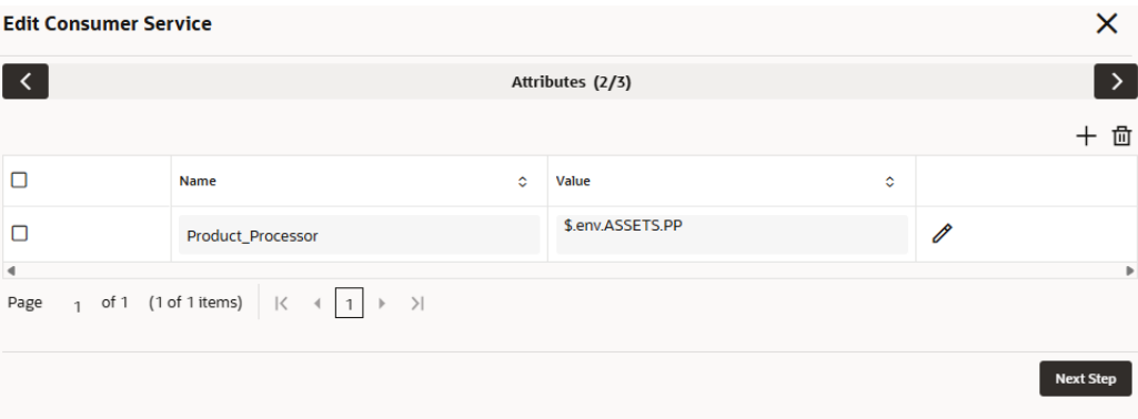
Figure 1-13 Add Attribute
