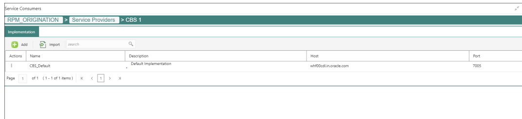
Figure 1-2 RPM_ORIGINATION - CBS
