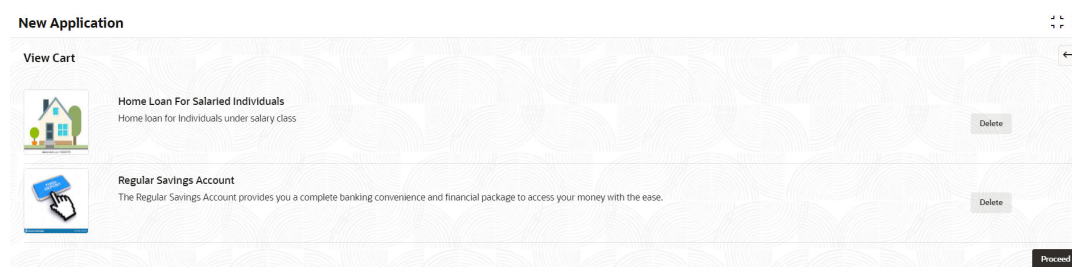
Figure 1-5 Cart Screen
