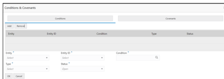
Figure 1-66 Conditions
