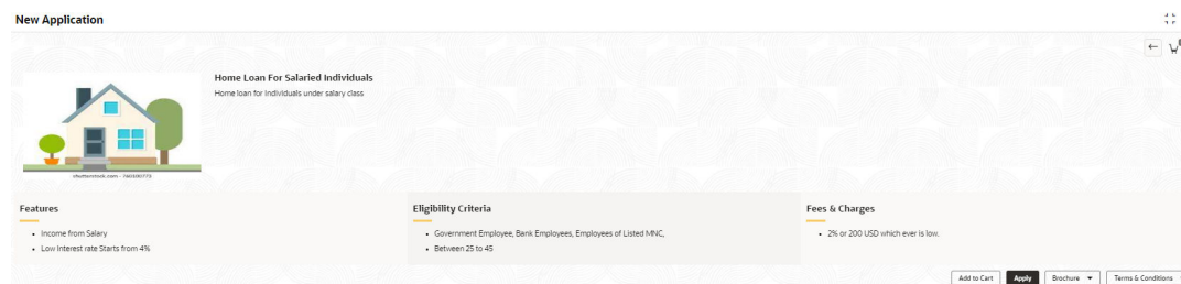
Figure 1-3 Product Details
