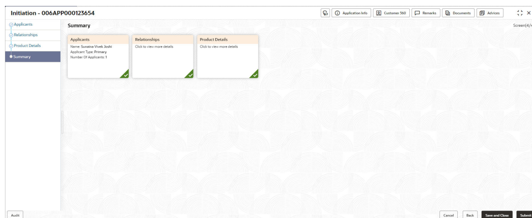
Figure 1-17 Summary
