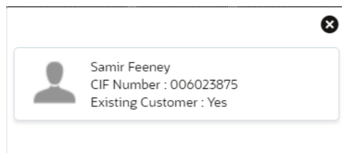
Figure 1-59 Customer 360
