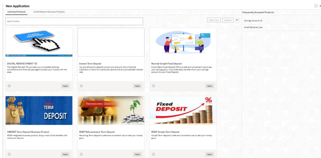
Figure 1-2 Product List
