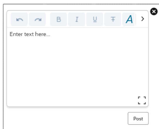
Figure 1-61 Remarks
