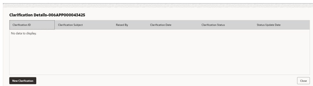
Figure 1-69 New Clarification
