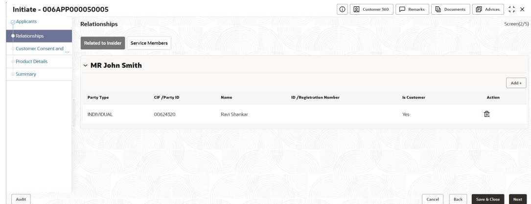
Figure 1-30 Relationships
