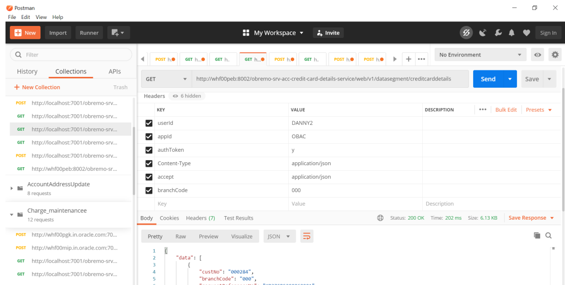
Figure 4-12 Postman
