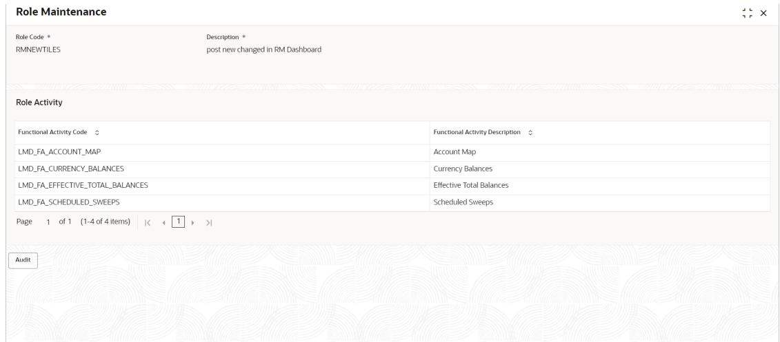
Figure 4-5 Role Maintenance
