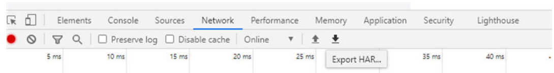
Figure 1-4 Export Option
