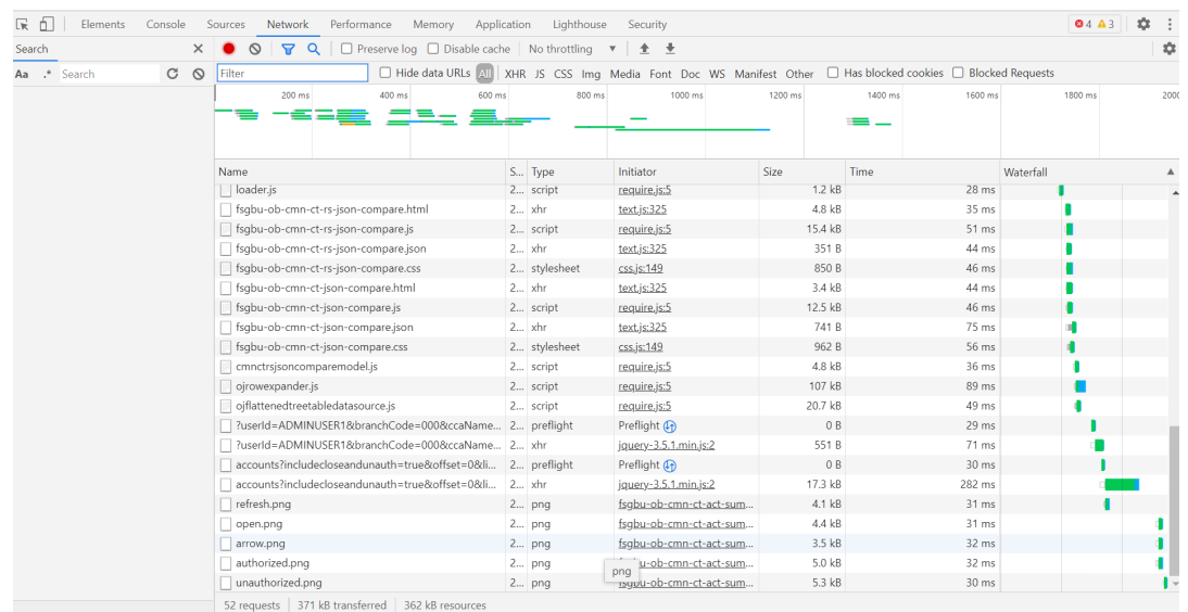
Figure 1-2 Call Responses
