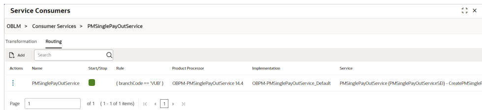
Figure 1-11 Routing Menu
