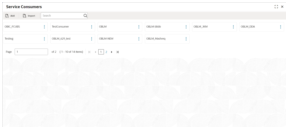
Figure 1-5 Consumer OBLM
