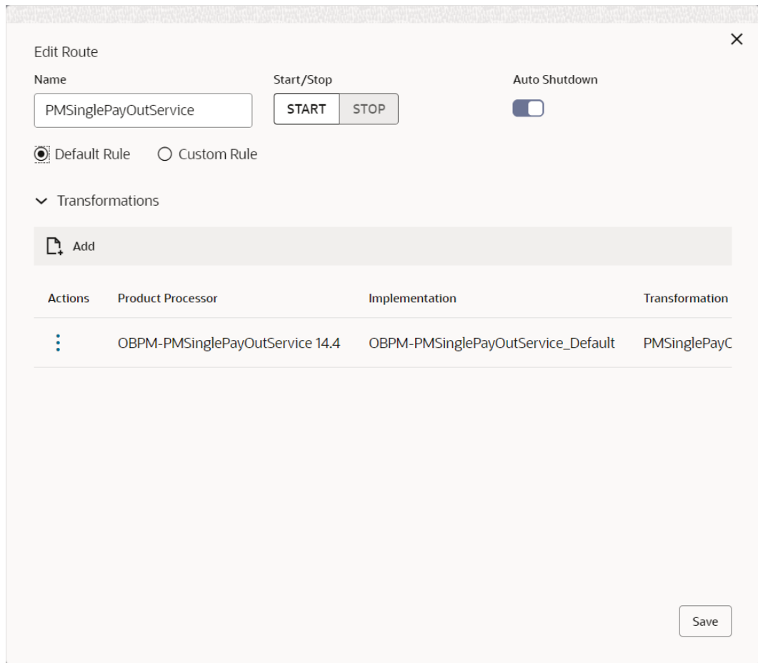
Figure 1-12 Edit Route
