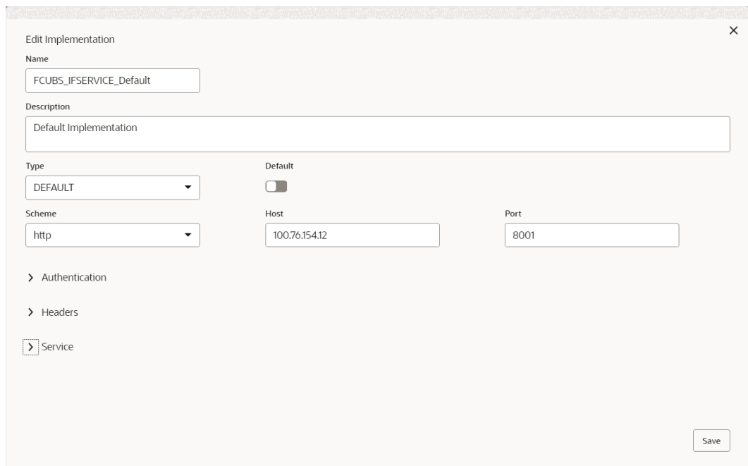
Figure 1-8 Edit Implementation
