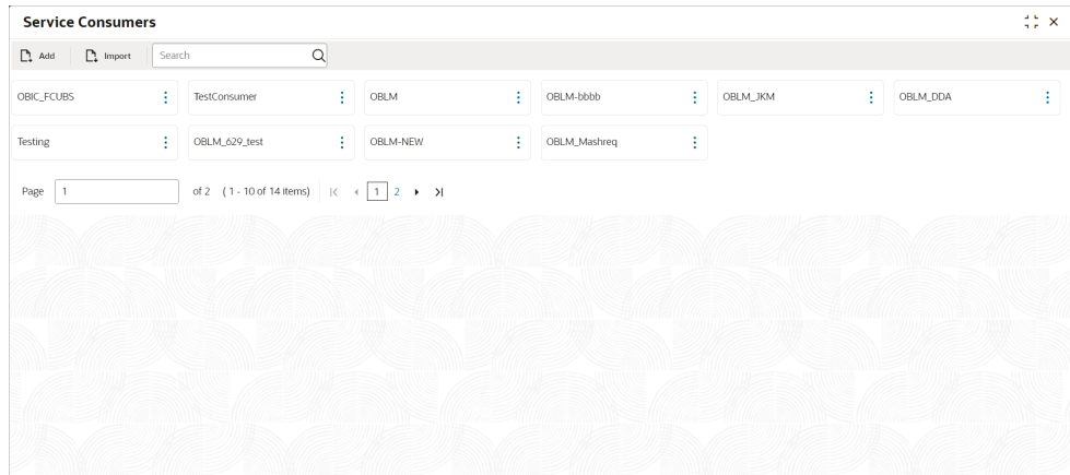
Figure 1-9 Consumer OBLM
