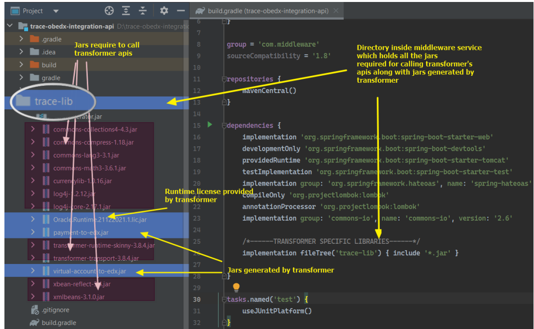
Figure 1-1 Middleware service
