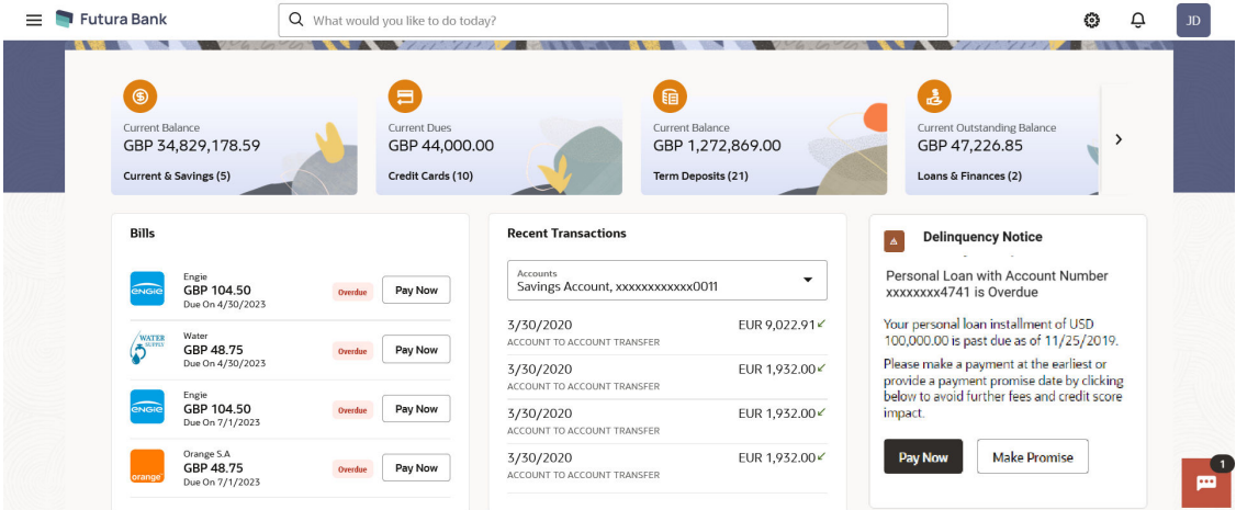
Figure 1-1 Overview widget
