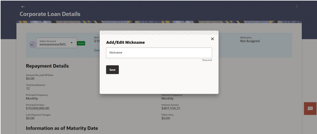
Figure 10-2 Add Nickname
