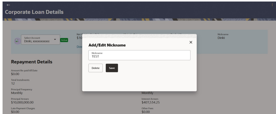
Figure 10-3 Edit Nickname
