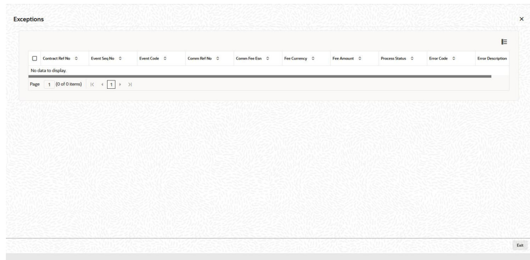
Figure 4-11 Exceptions
