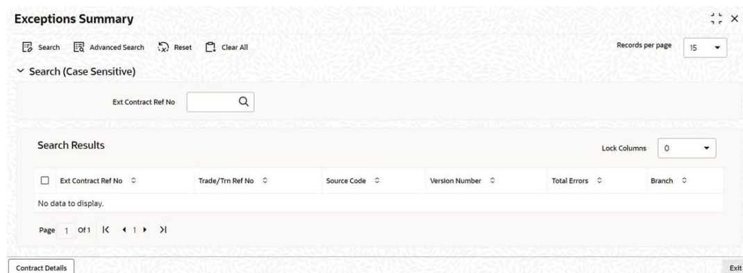
Figure 4-3 Exceptions Summary
