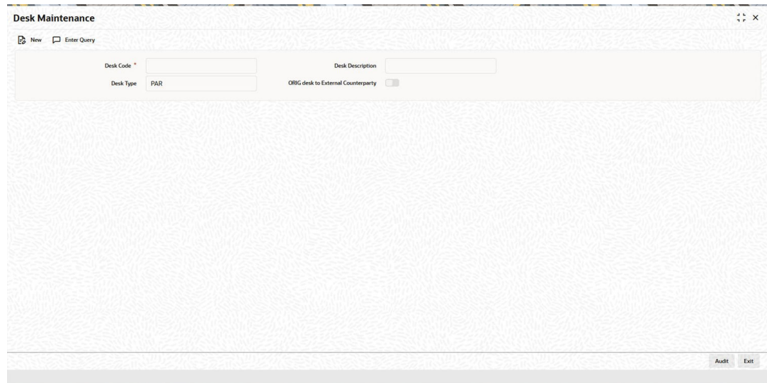
Figure 2-2 Desk Maintenance
