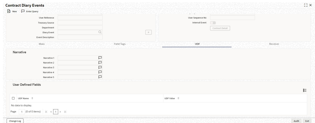
Figure 2-7 UDF
