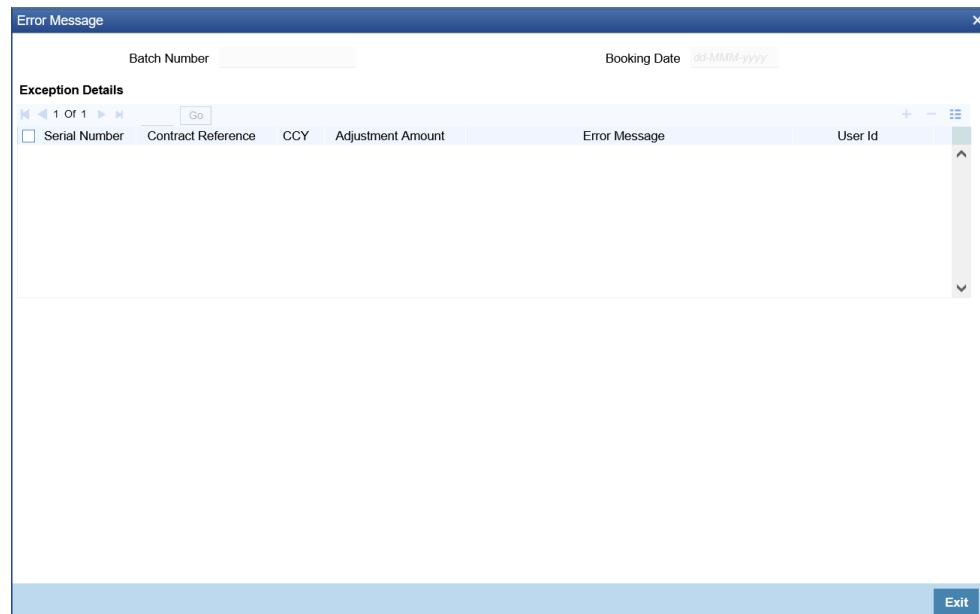
Figure 4-18 Error Message
