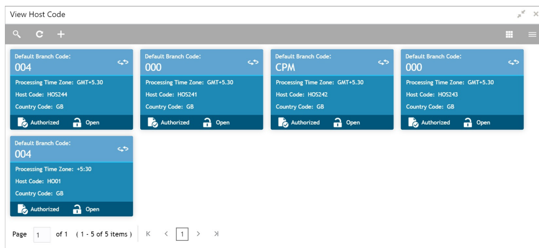
Figure 1-7 Tile View
