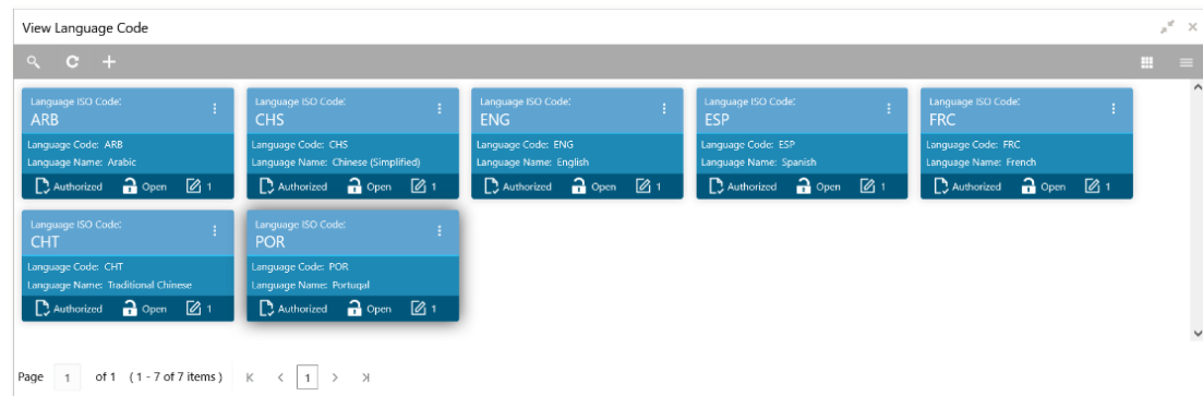
Figure 1-5 Summary Screen
