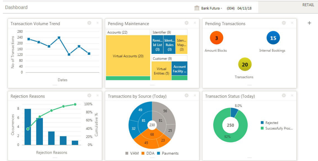
Figure 1-4 Dashboard
