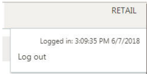
Figure 1-2 User Profile
