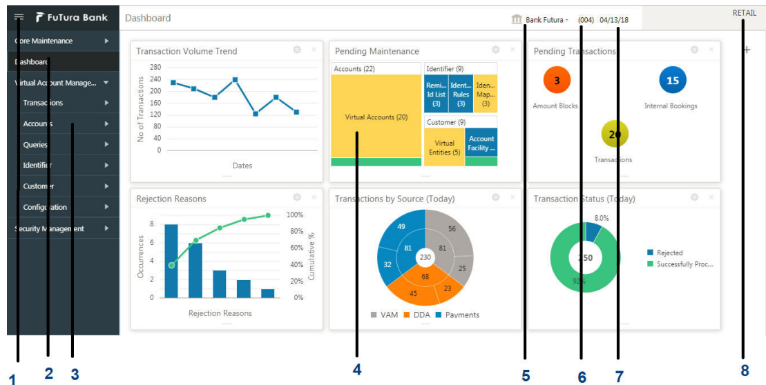
Figure 1-3 Application Environment
