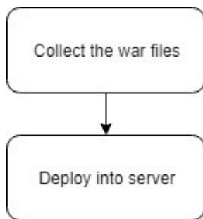
Figure 5-1 Deployments
