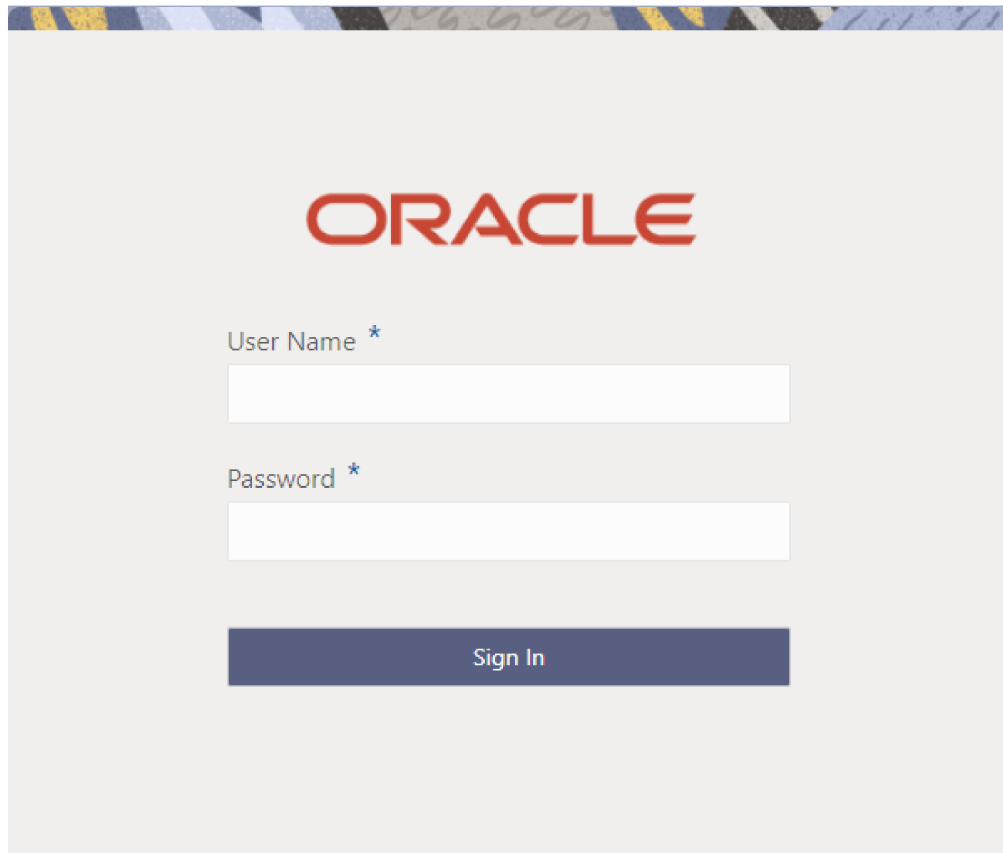
Figure 1-6 Login Page
