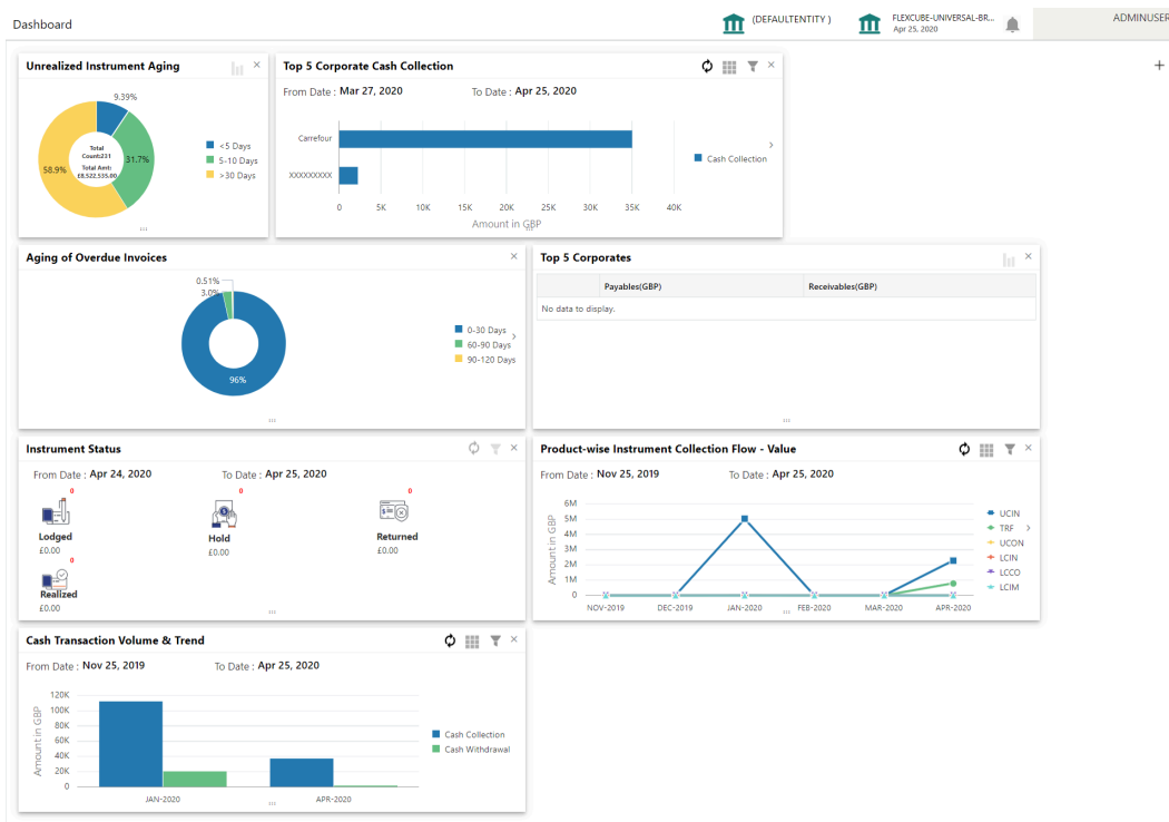
Figure 1-2 Dashboard
