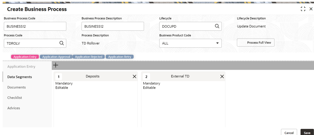
Figure 3-4 Create Business Process - Added Data Segments
