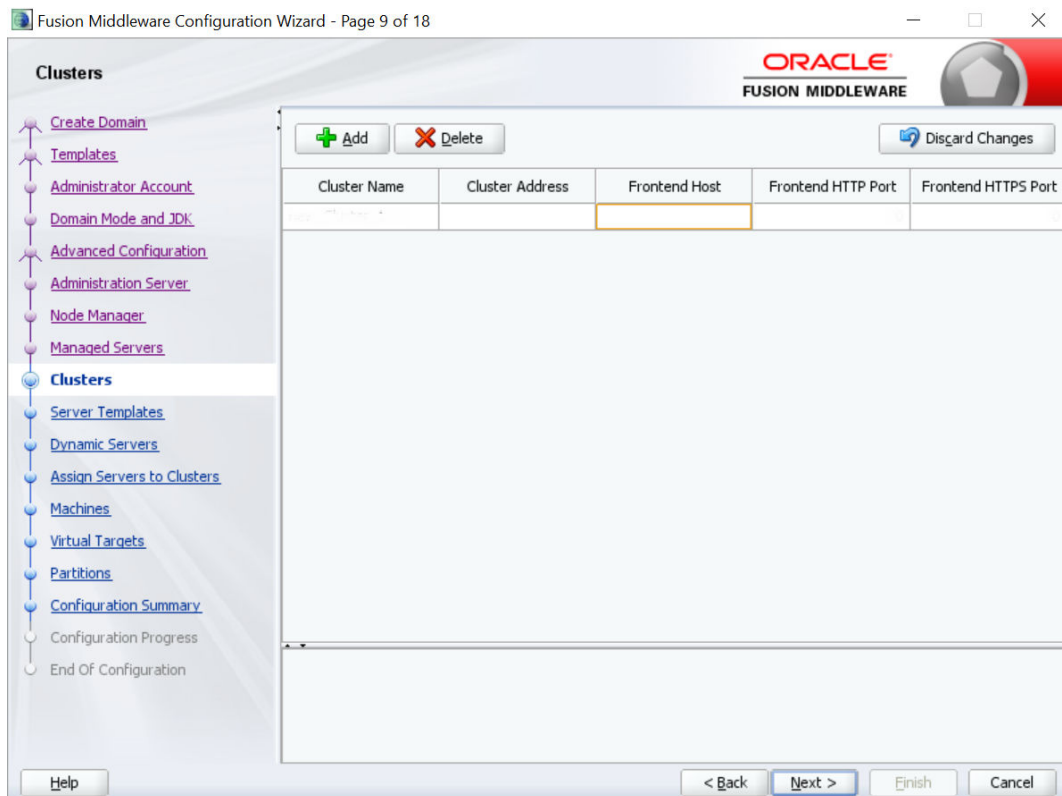
Figure 11-4 Clusters
