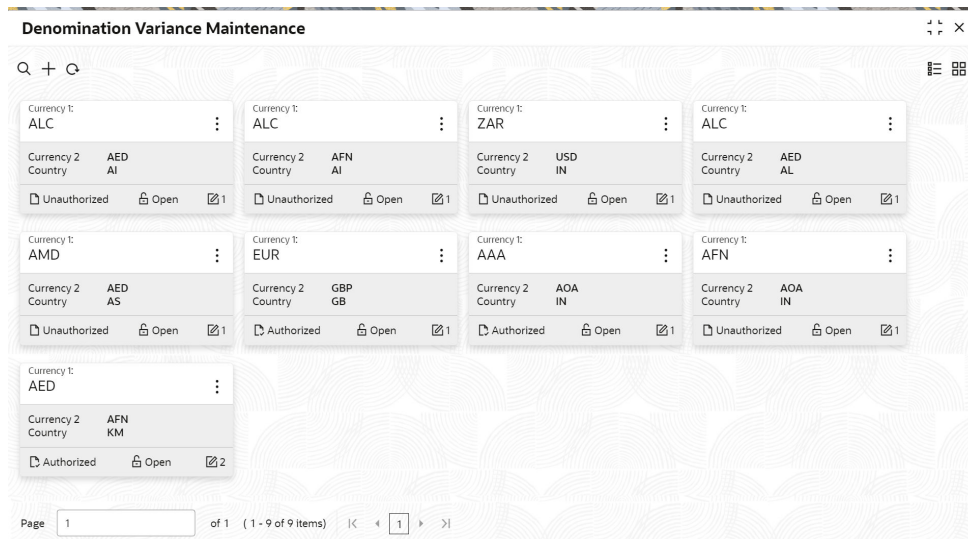
Figure 20-46 Denomination Variation Maintenance (Summary)
