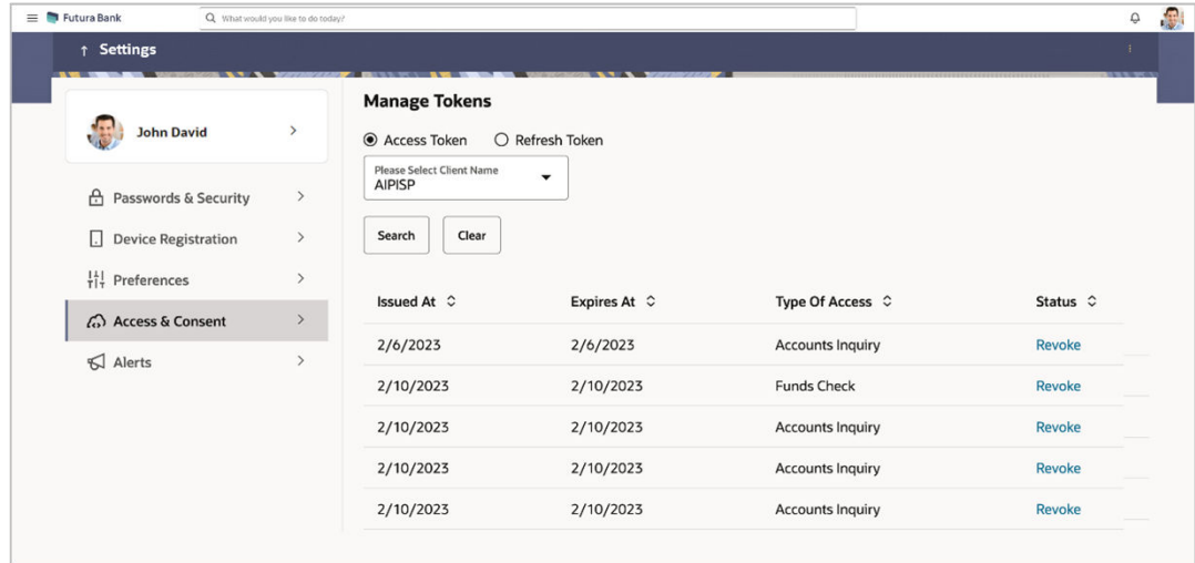
Figure 2-8 Manage Tokens
