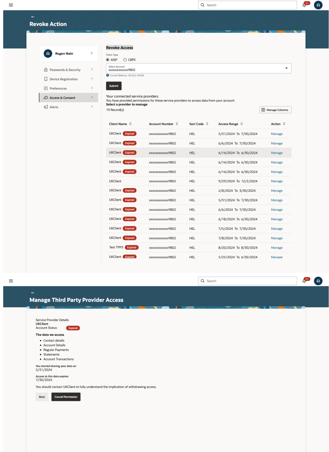
Figure 2-7 Revoke Access
