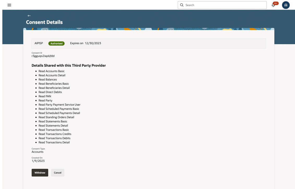
Figure 2-6 Consent Revocation
