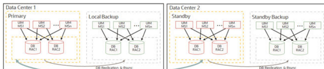
Figure 14-4 UIM Cloud Native Deployment and the Associated RAC Database
