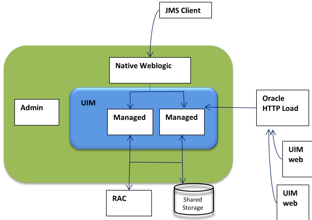
Figure 14-1 UIM Single-Site High Availability Architecture
