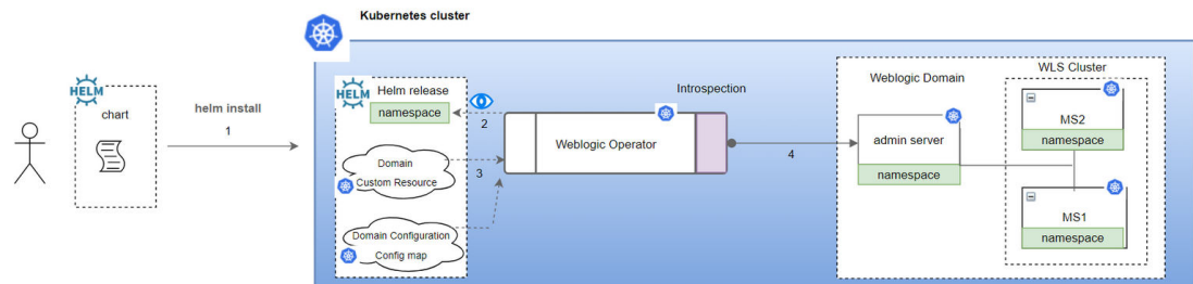
Figure 1-2 UIM Cloud Native Deployment Environment
