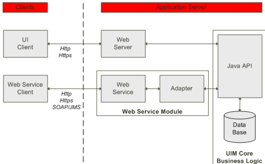
Figure 1-1 UIM Web Services
