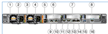
Figure 1-2 Device Back Panel
