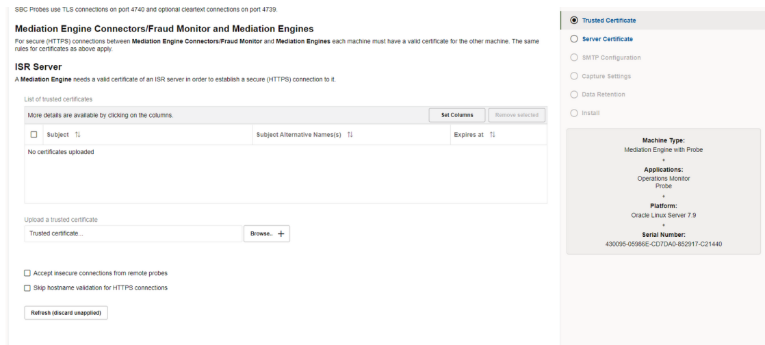
Figure 4-6 Trusted Certificate page
