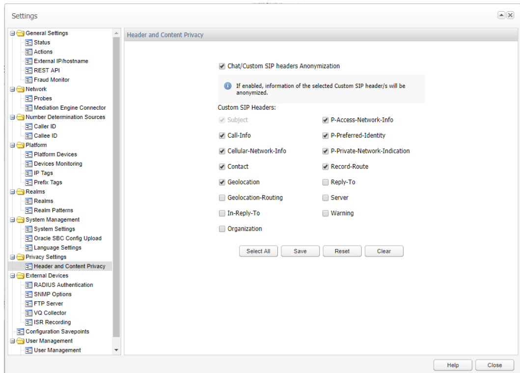
Figure 7-33 Header and Content Privacy
