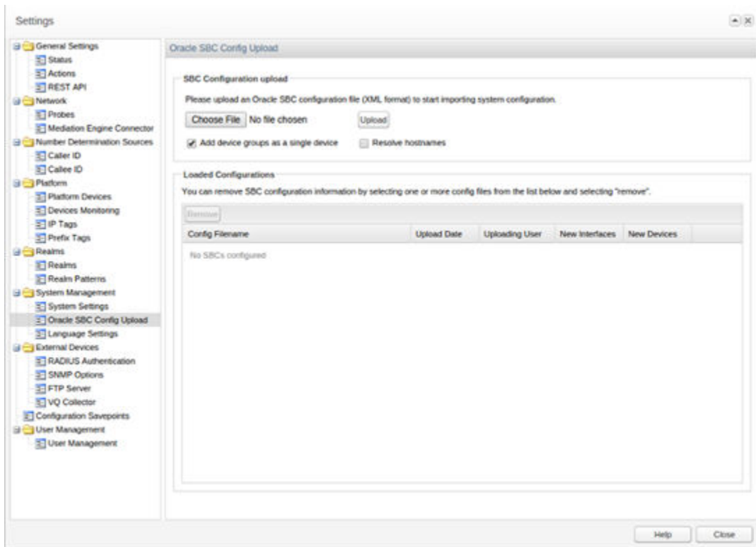
Figure 7-30 Oracle SBC Config Upload Page
