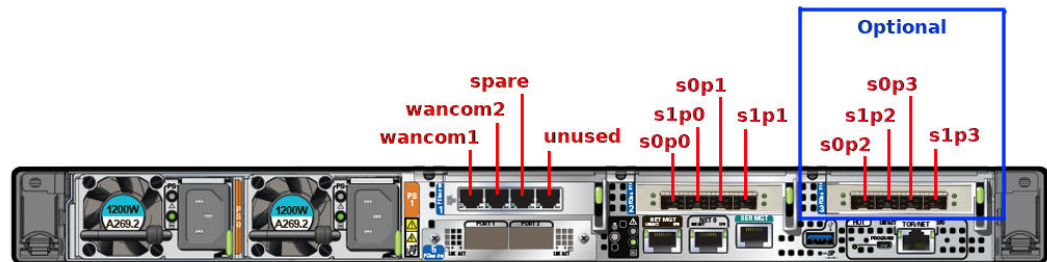
Figure 5-11 Oracle Server X9-2 Configuration B: four-port 10-Gigabit QSFP+ NIC
