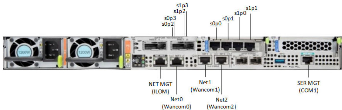
Figure 4-13 Oracle X8-2 Configuration B (One QSFP and One 4x10 GigE NICs)
