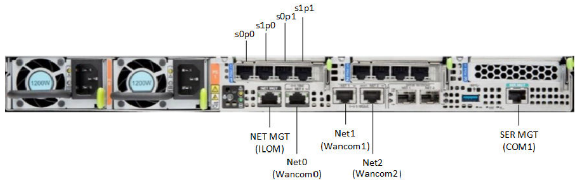
Figure 4-11 Oracle X8-2 Configuration A (4x10 GigE NIC)
