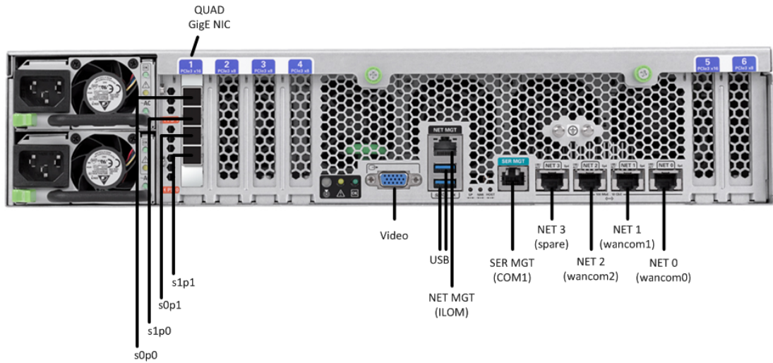
Figure 2-2 Netra X5-2 for Communications Configuration B (4 Onboard 10 Gig Ports & 1 Quad GigE NIC)
