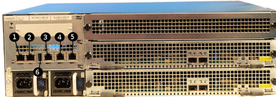
Figure A-6 Acme Packet 6300/6350 Management Interfaces
