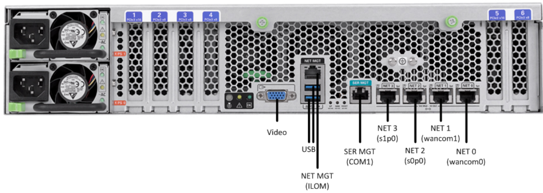
Figure 2-2 Netra X5-2 for Communications Configuration B (4 Onboard 10 Gig Ports & 1 Quad GigE NIC)
