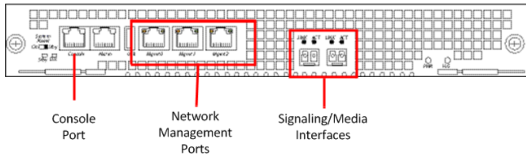
Figure A-4 Acme Packet 6100 - Rear View
