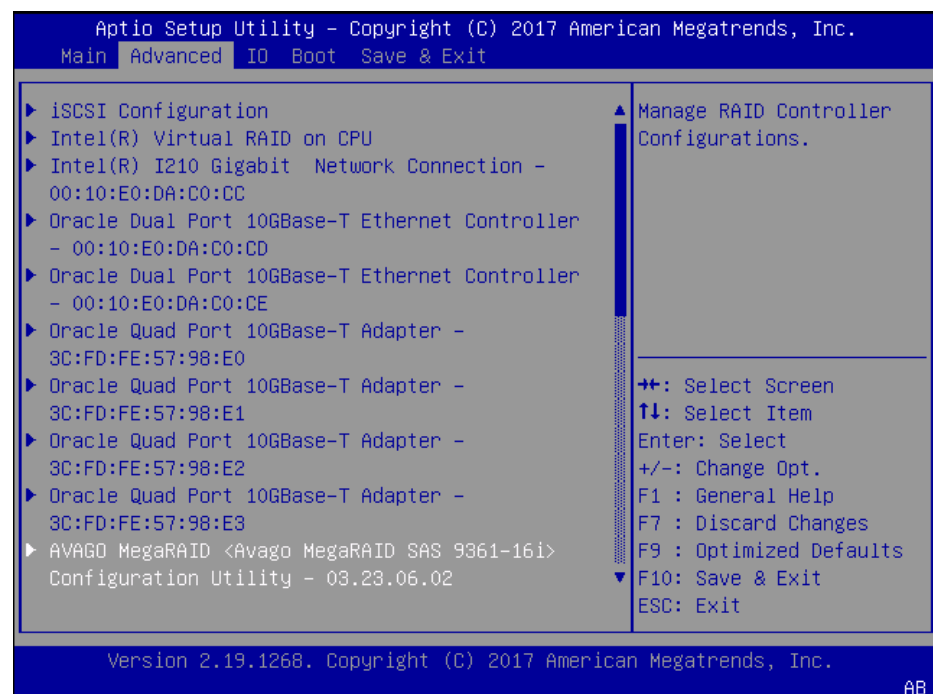
Figure 4-1 Selecting RAID Configuration
