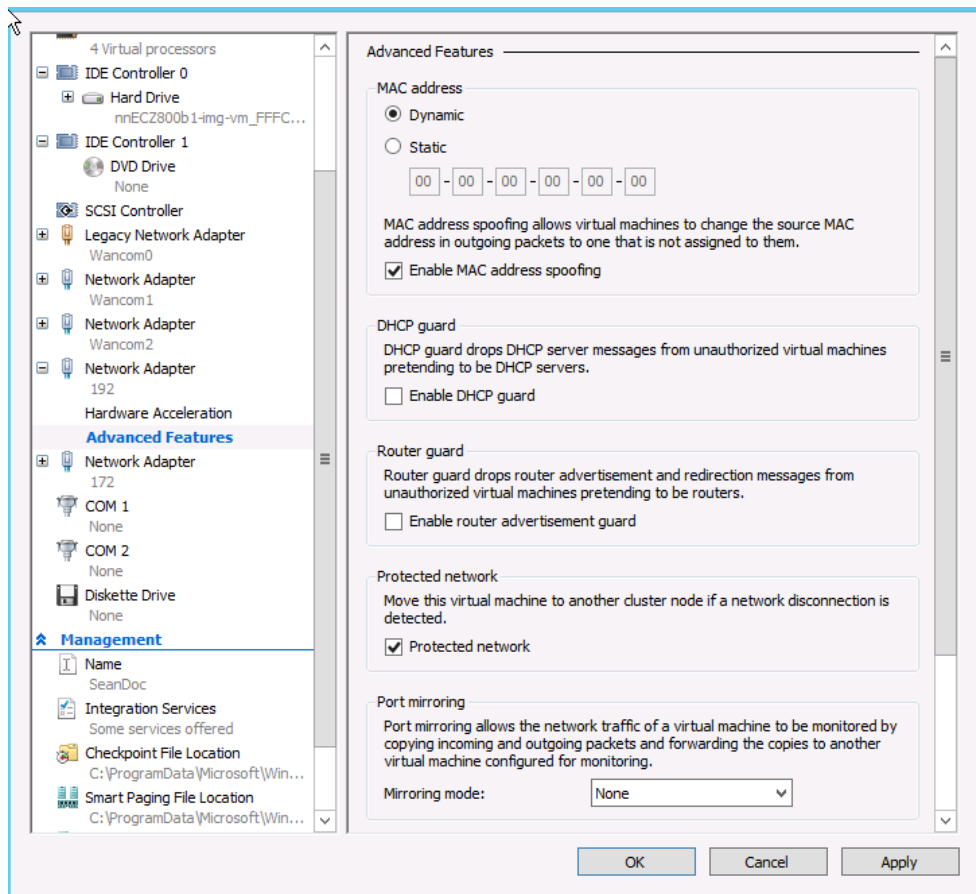
Figure 6-1 VM Settings on Hyper-V
