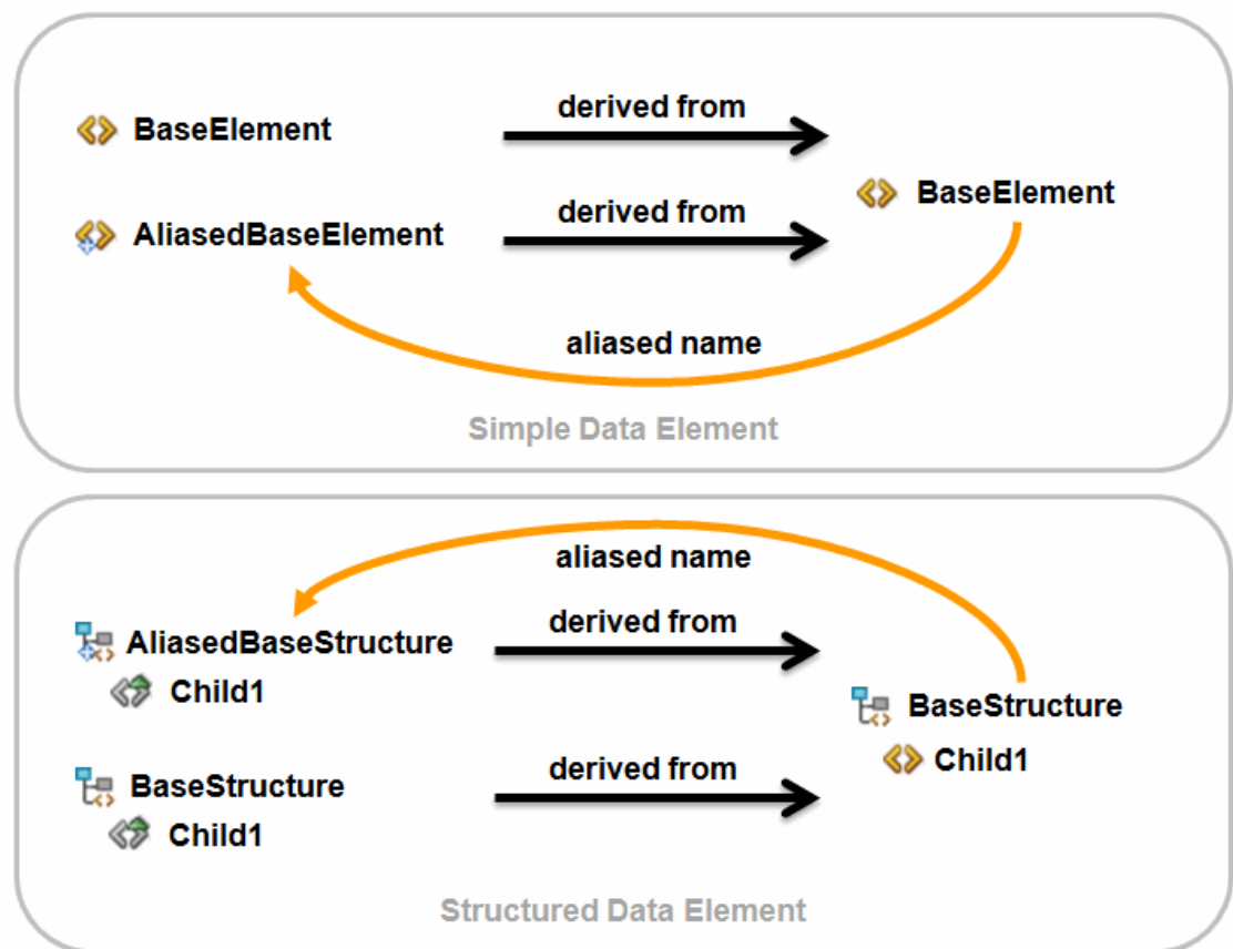
Figure 4-7 Aliased Data Elements
