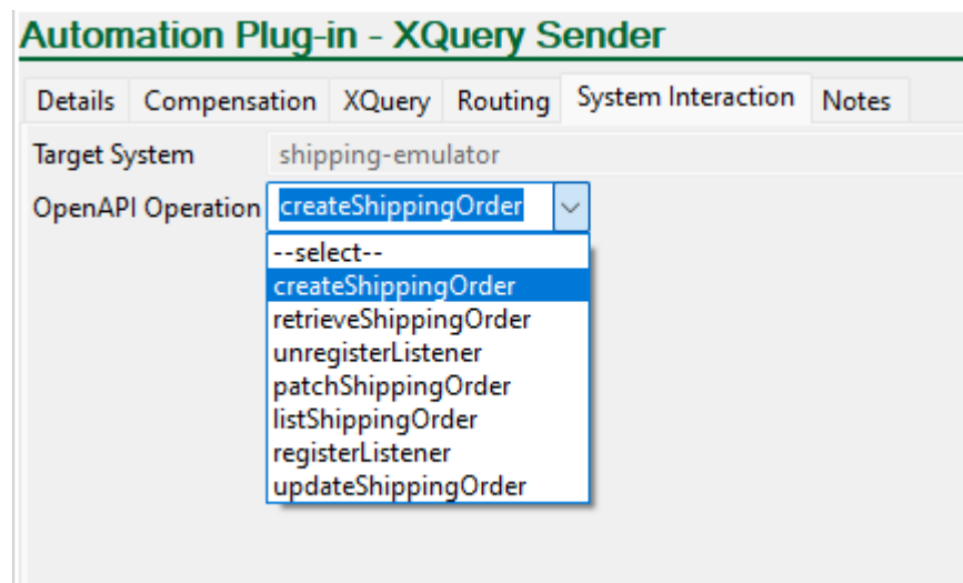
Figure 12-1 SI Operations Dropdown
