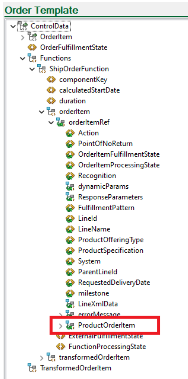
Figure 11-4 ProductOrderItem within a Function
