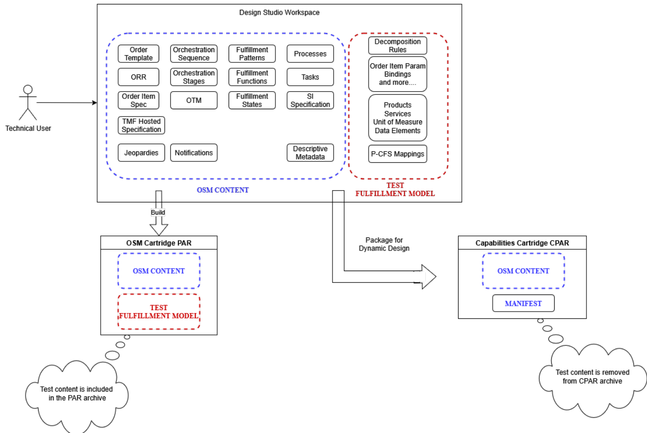
Figure 20-9 Test Data During Design Journeys
