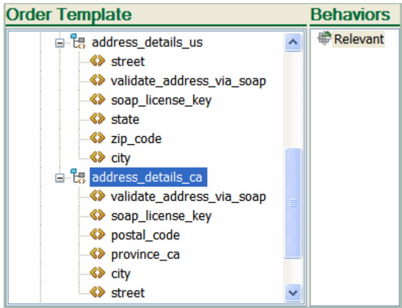
Figure 9-6 Address Fields in Design Studio
