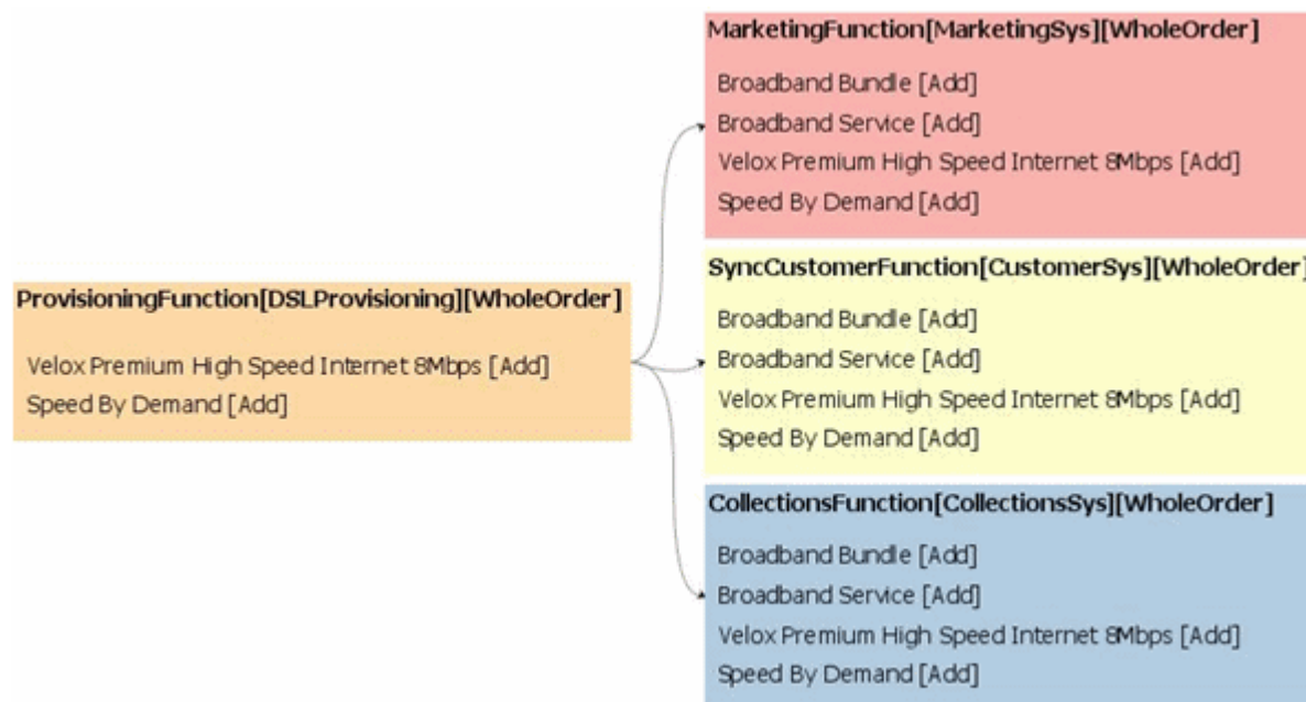
Figure 5-23 Inferred Dependencies at Run Time
