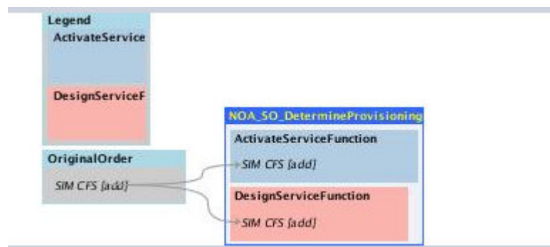
Figure 12-3 activationOrchPlan
