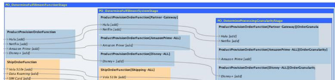
Figure 12-4 digitaltv
