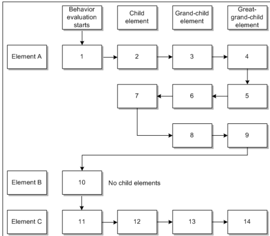
Figure 9-3 Element Selection
