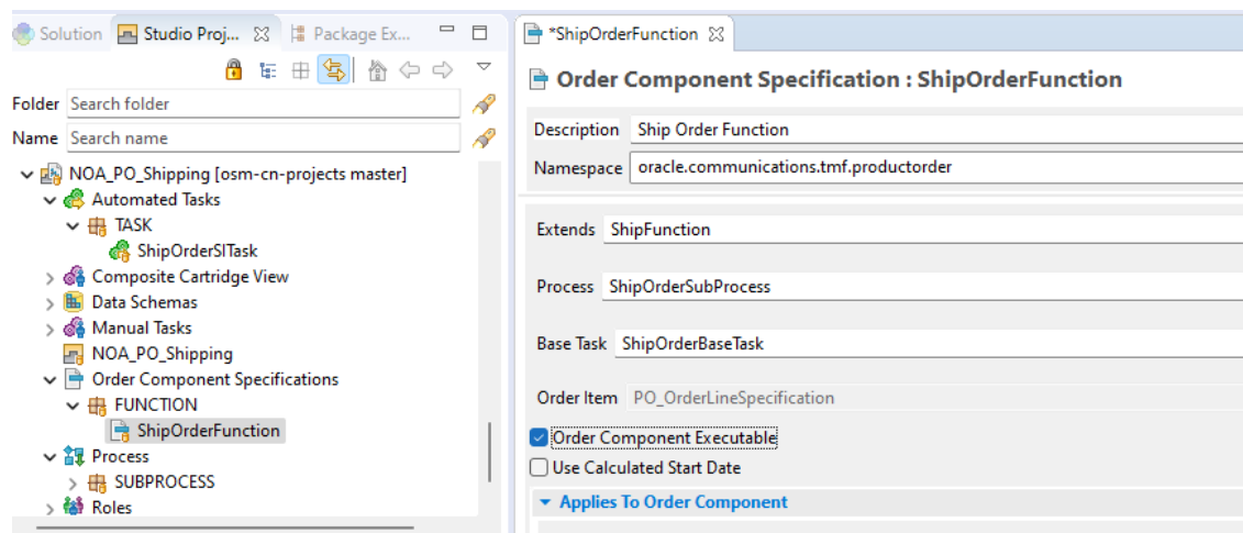
Figure 12-2 ShipOrderSubProcess
