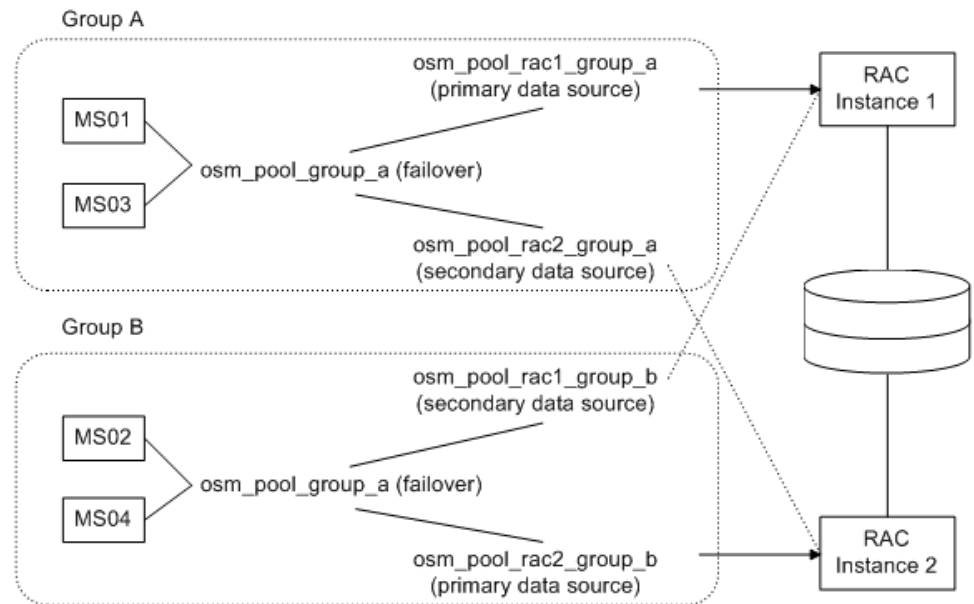
Figure 6-2 OSM Data Source Configuration for Active-Active Oracle RAC
