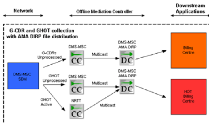
Figure 12-3 AMA Architecture with G-CDR and GHOT Collection in AMA DIRP File Format
