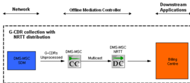
Figure 12-2 AMA Architecture with G-CDR Collection in NRTT Distribution
