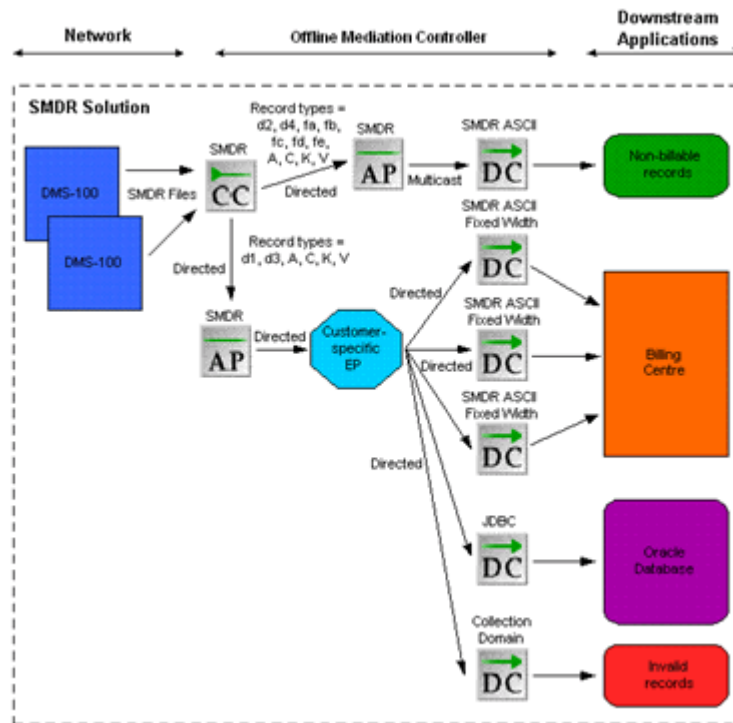
Figure 11-1 SMDR Solution
