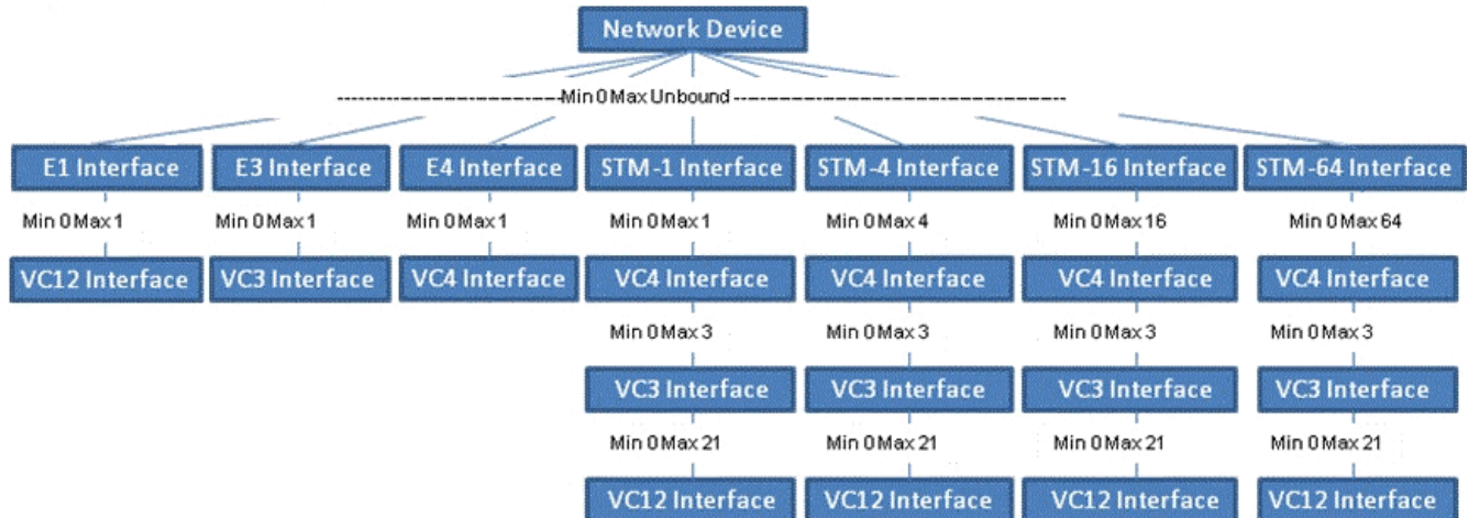
Figure 7-1 Logical Specification Lineage
