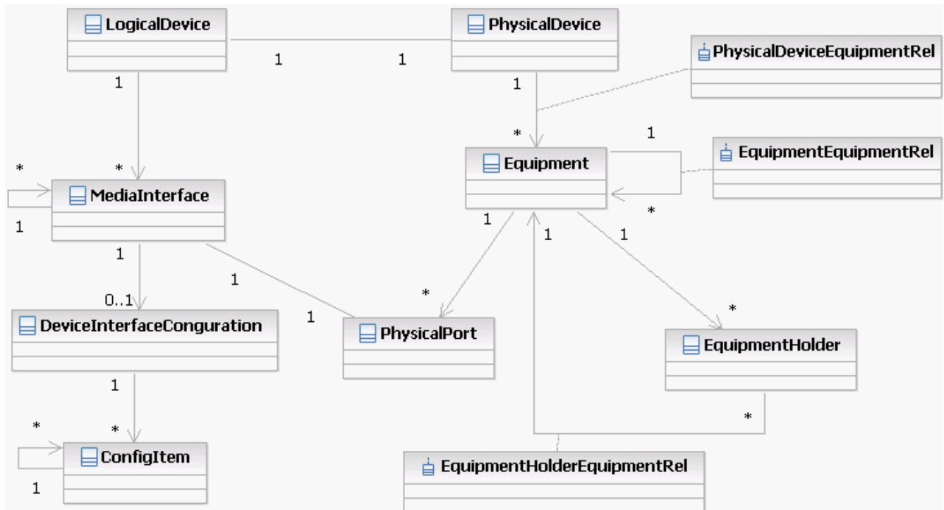
Figure 5-1 Generic SNMP Cartridge UML Representation
