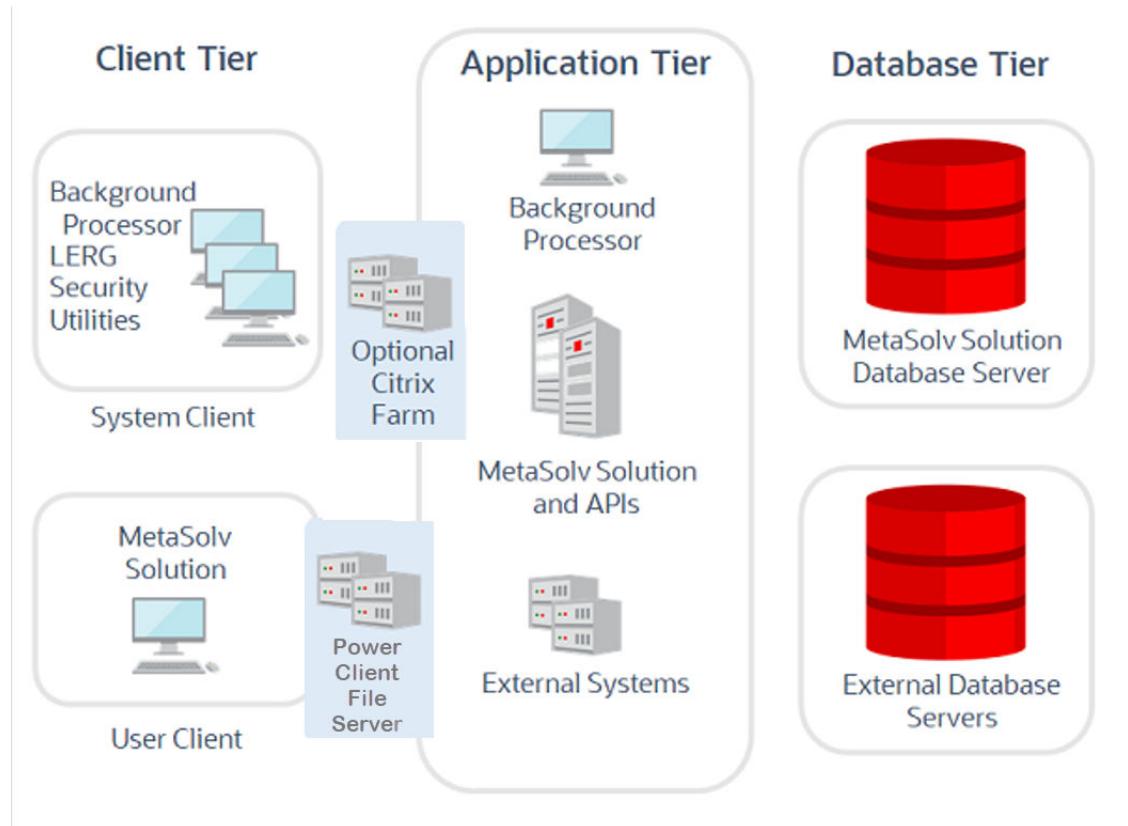
Figure 1-1 MetaSolv Solution Three-Tier Architecture
