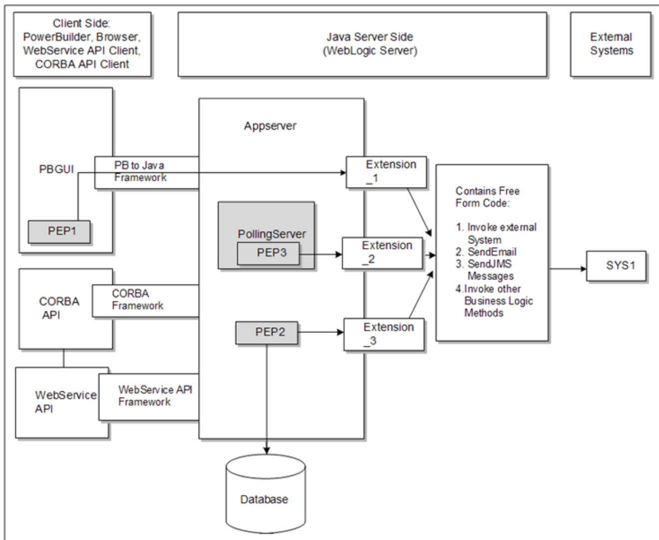
Figure 1-1 Architecture Supporting Extension Functionality
