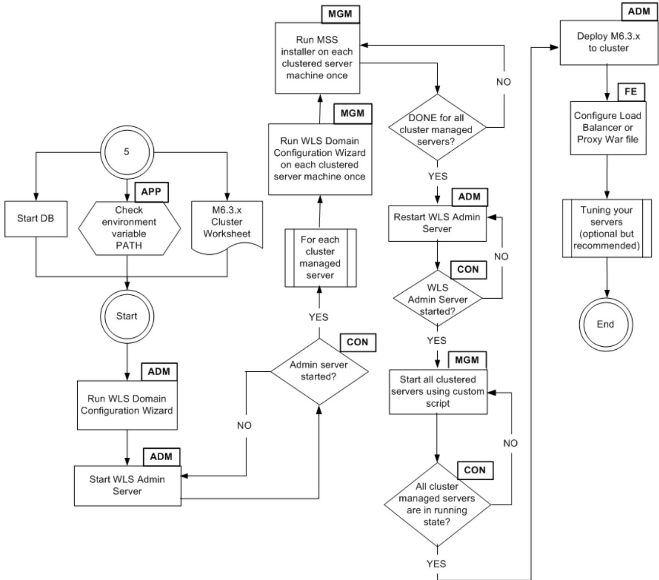
Figure 5-1 Installing a Cluster-Managed Server
