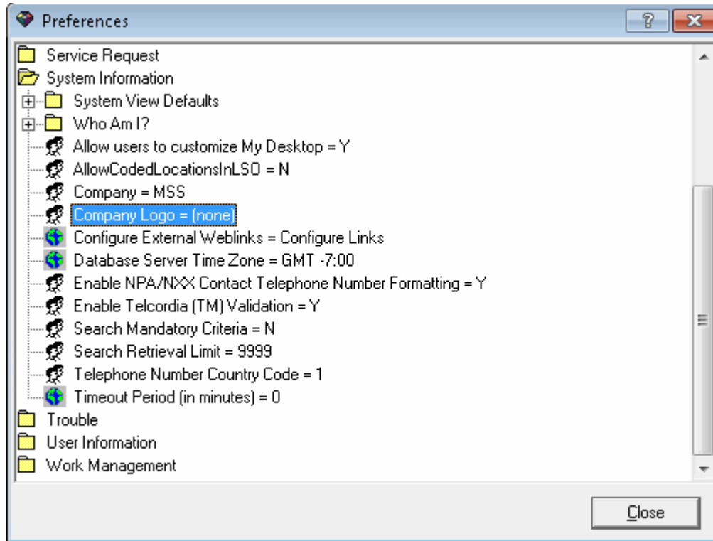
Figure 8-2 Preferences Window
