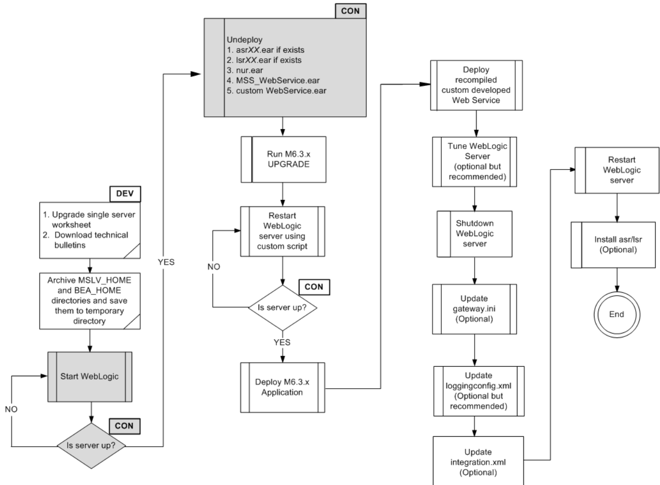
Figure 6-4 Undeploying Applications
