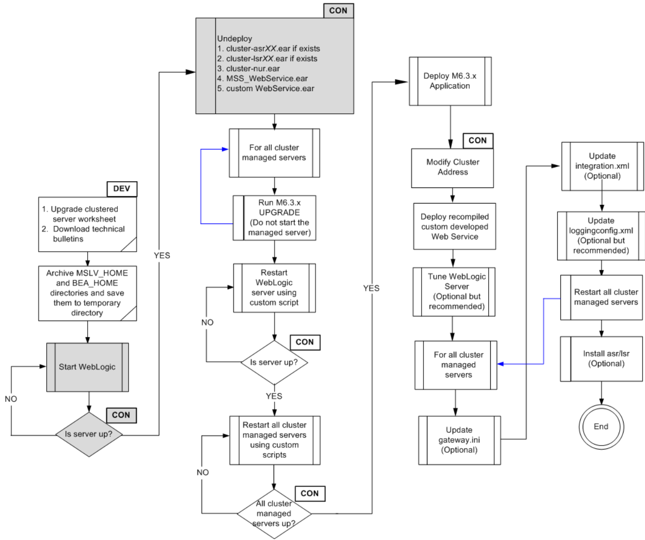
Figure 6-9 Undeploying Applications
