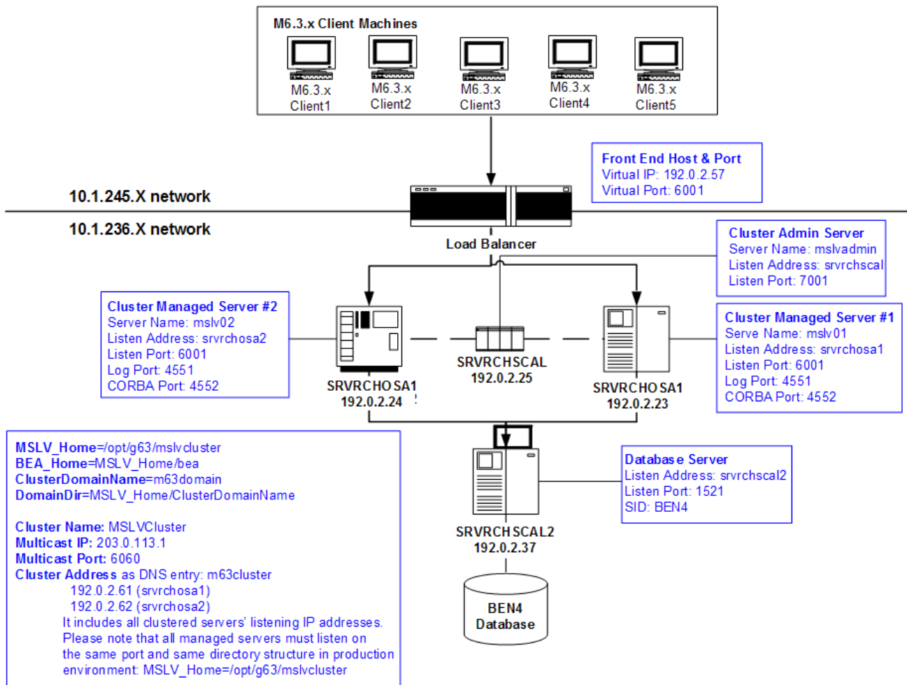
Figure 5-2 Example Cluster-Managed Server Configuration
