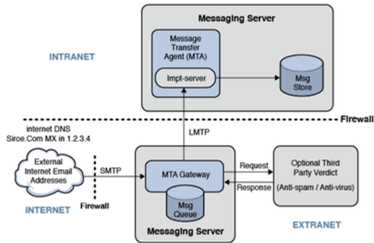
Figure 63-7 How a User Receives Email from the MTA
