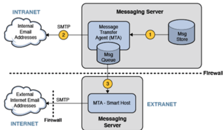
Figure 63-6 How the MTA Delivers a Message
