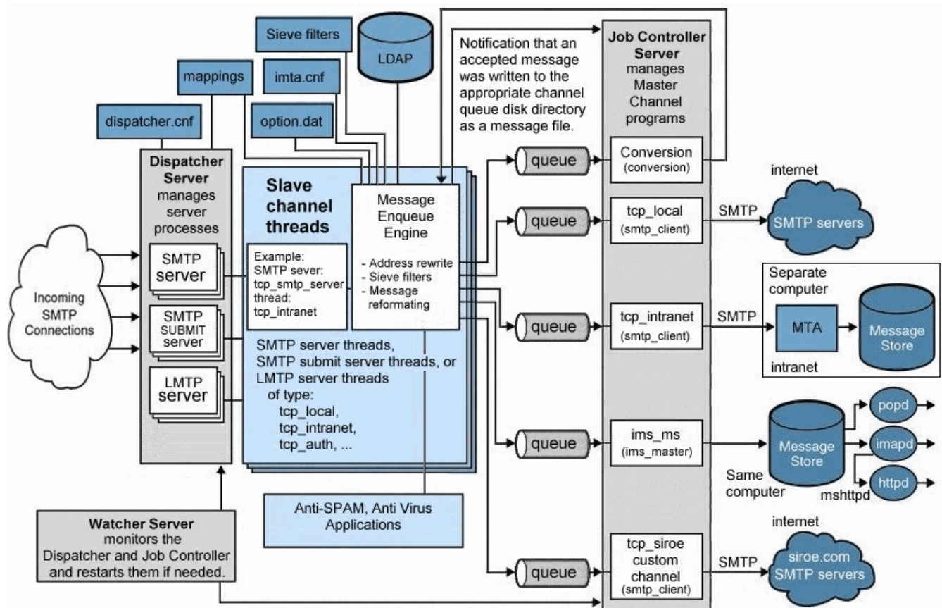
Figure 6-2 MTA Architecture
