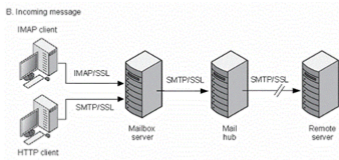
Figure 7-2 Incoming Encrypted Communications with Messaging Server
