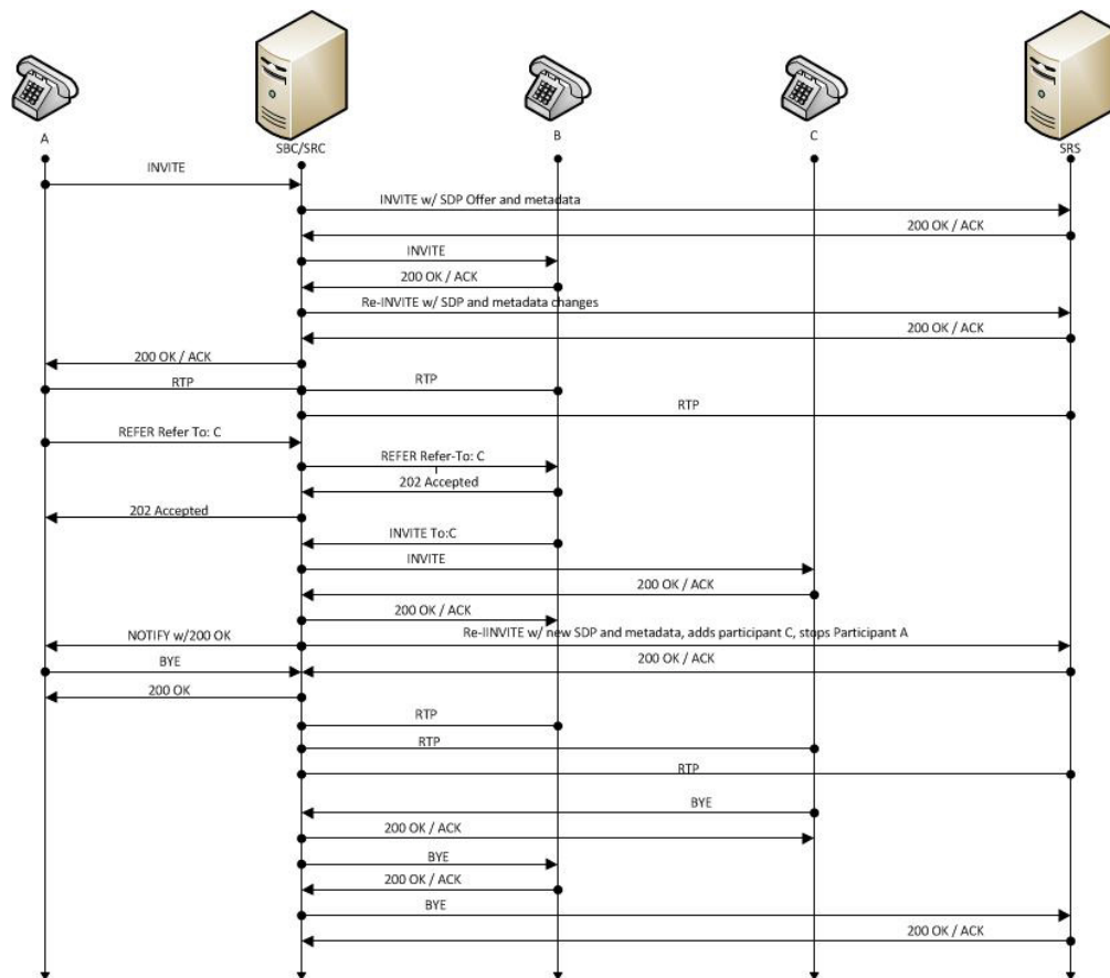
SIP REFER, UA handles REFER, "recording required", selective recording
