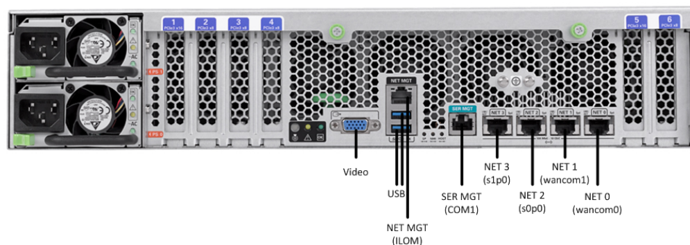
Figure 1-31 Netra X5-2 for Communications Configuration A (4 Onboard 10 GigE Ports)
