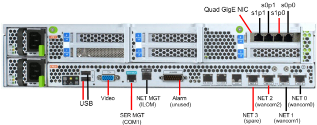
Netra Server X3-2 for Acme Packet Configuration B (4 Onboard 10 GigE Ports & 1 Quad GigE NIC)
