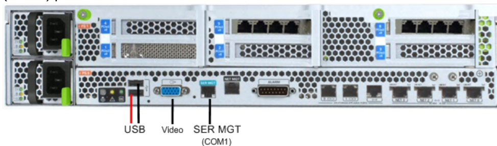
Connecting to USB, VGA and SER MGT (COM1) Ports
