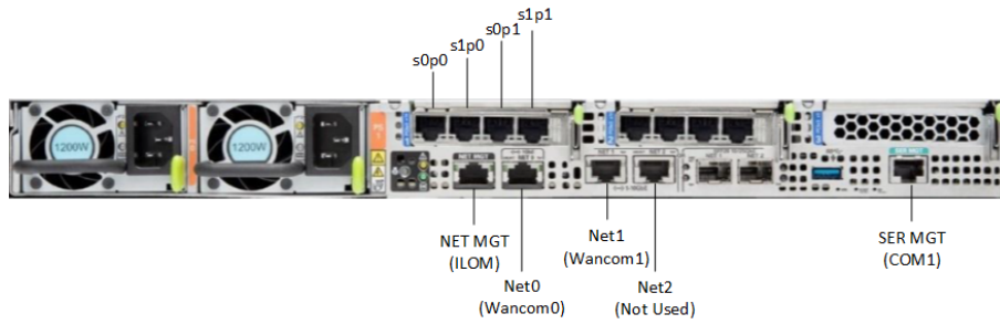
Figure 1-11 Oracle X8-2 Configuration A (4x10 GigE NIC)
