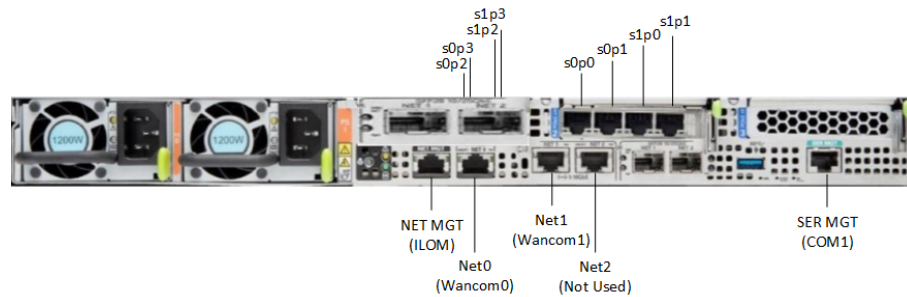
Figure 1-13 Oracle X8-2 Configuration B (One QSFP and One 4x10 GigE NICs)
