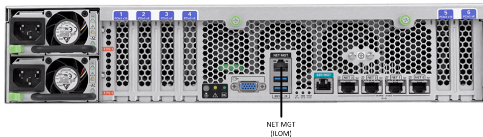
Figure 1-35 Connecting to ILOM Port
