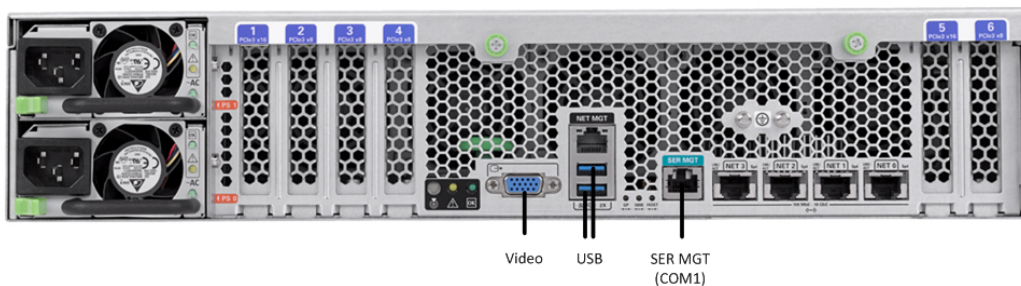
Figure 1-34 Connecting to USB, VGA and SER MGT (COM1) Ports
