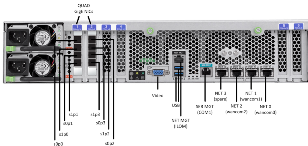
Figure 1-33 Netra 5-2 for Communications Configuration C (4 Onboard 10 GigE Ports & 2 Quad GigE NICs)
