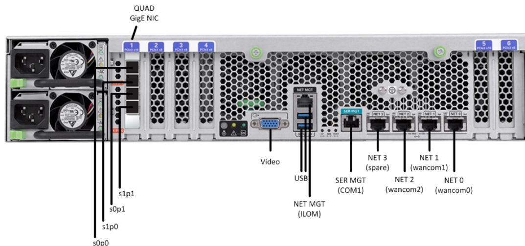
Figure 1-32 Netra X5-2 for Communications Configuration B (4 Onboard 10 GigE Ports & 1 Quad GigE NIC)
