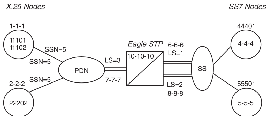
Figure 5-34 Gateway Network
