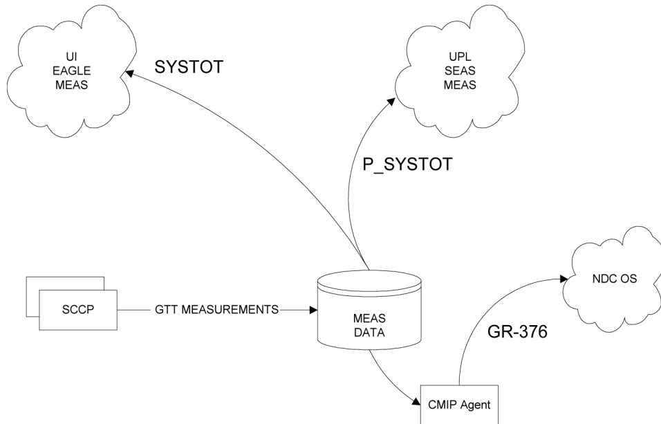
Figure 3-5 Concept Diagram
