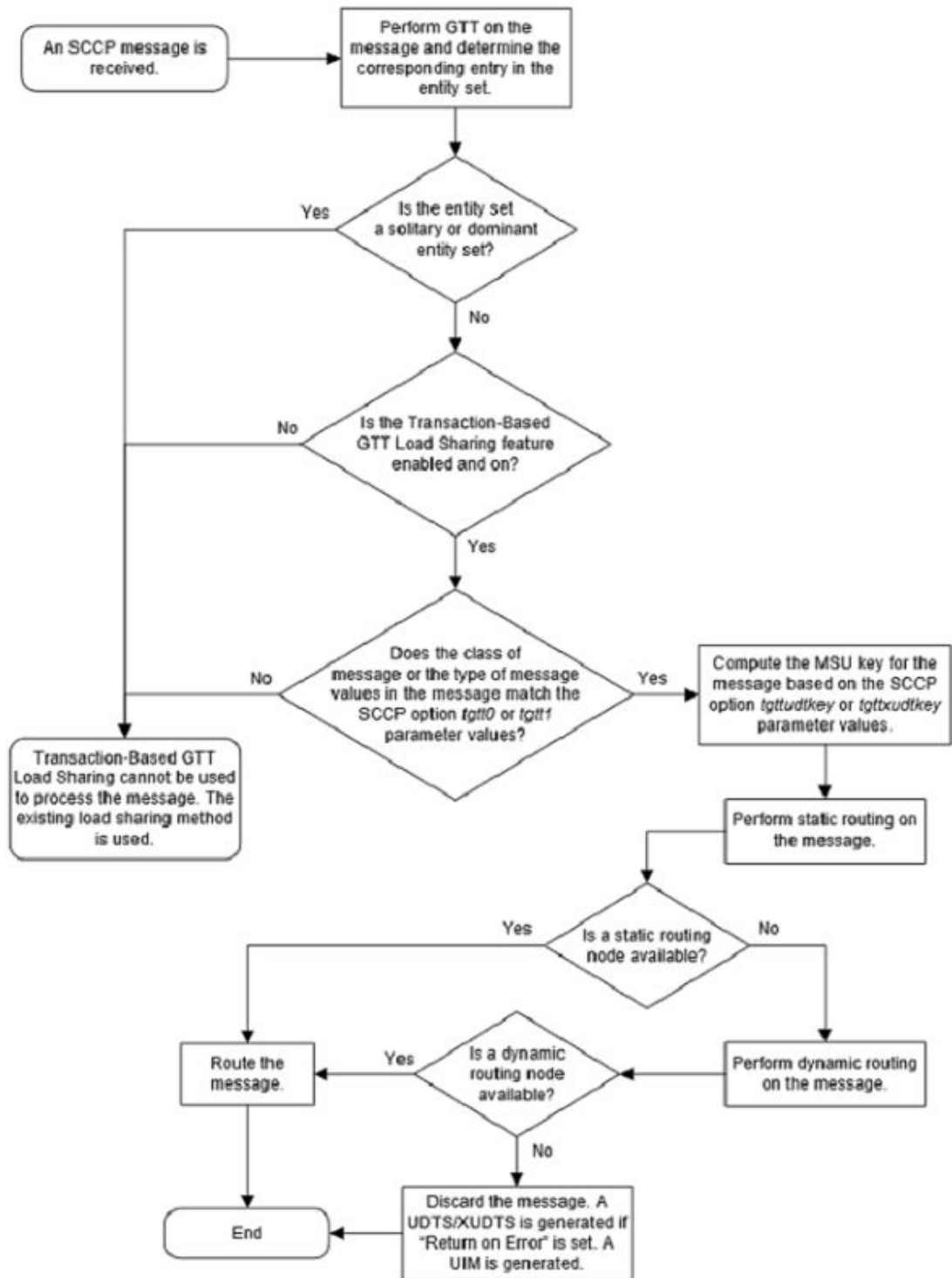
Figure 2-4 Message Routing using Transaction-Based GTT Load Sharing
