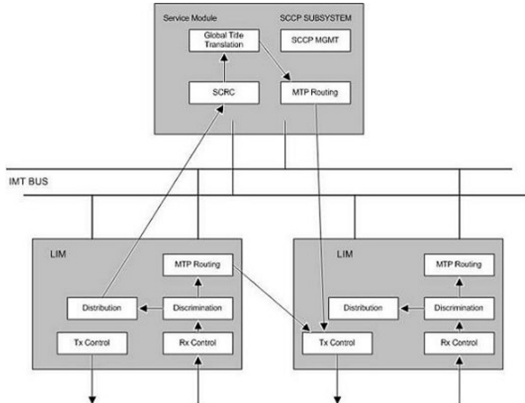
Figure 2-32 SCCP Message Flow through the EAGLE
