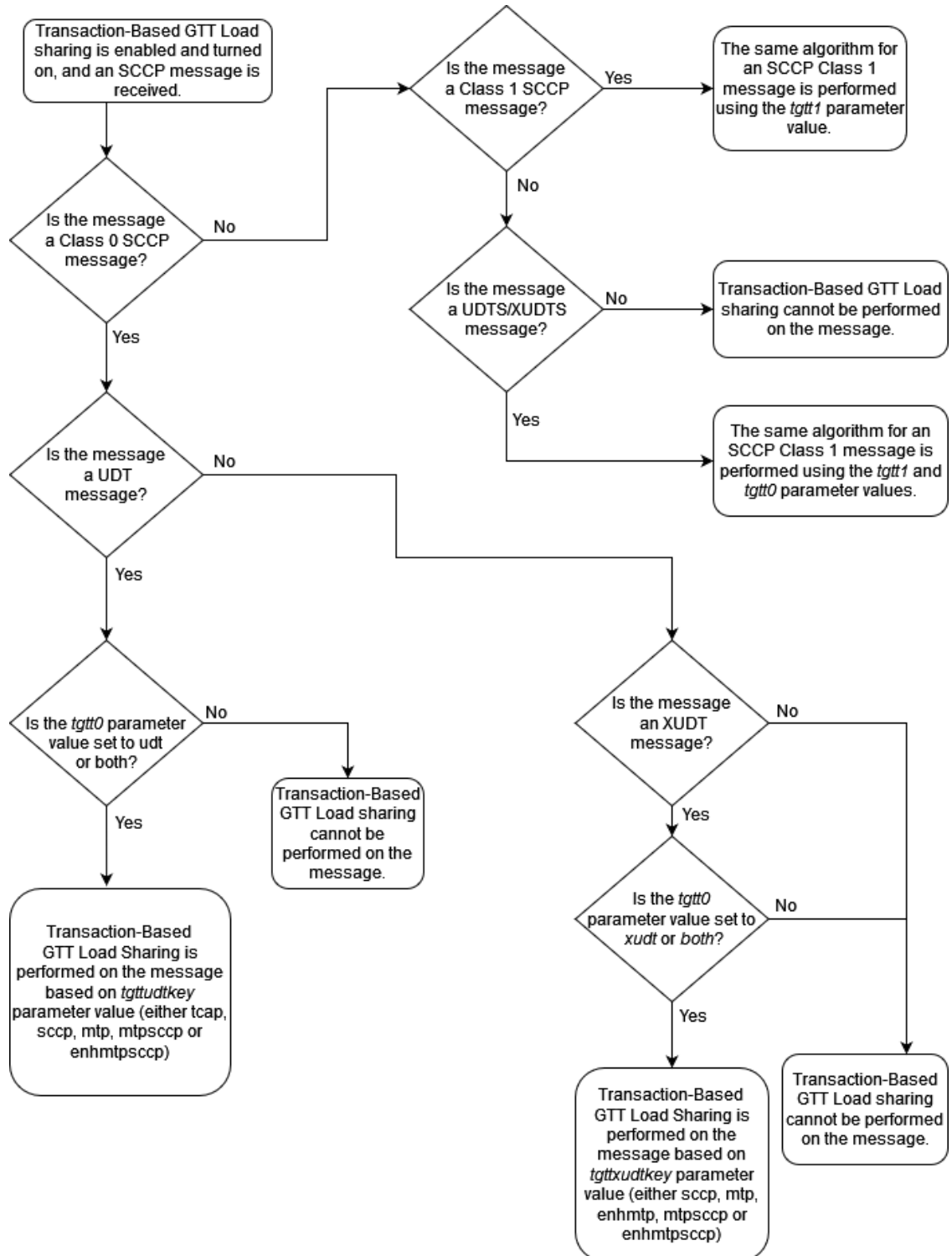
Figure 2-3 Transaction-based GTT Load Sharing SCCP Options
