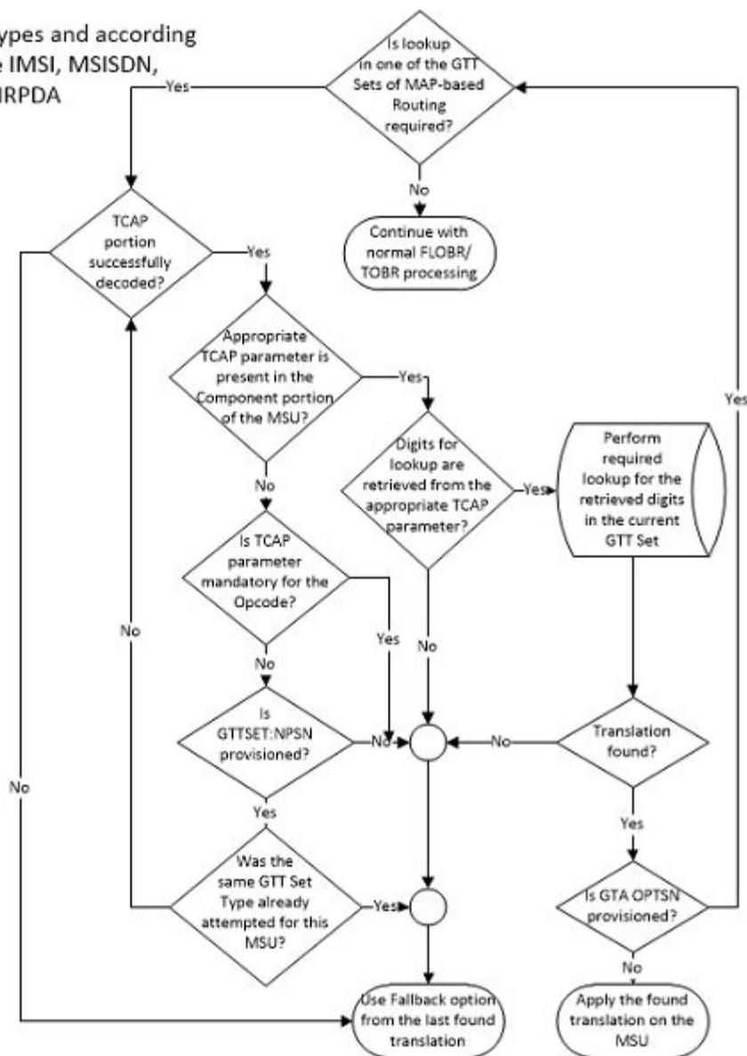
Figure 2-11 MAP Based Routing Flowchart
