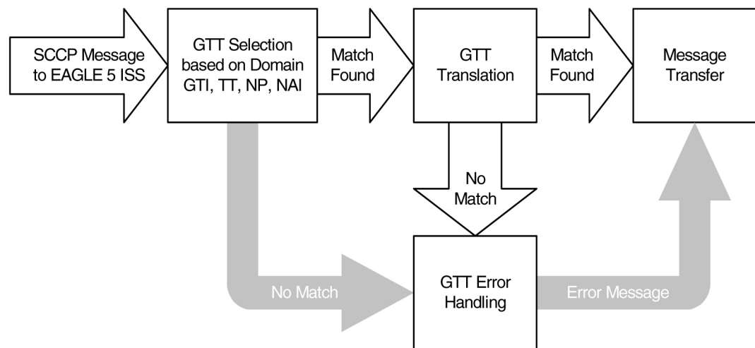
Figure 2-35 EGTT Process
