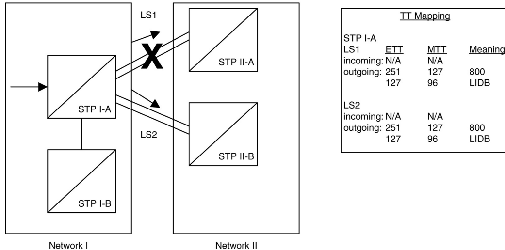
Figure 2-36 An Example of Double Translation Type Mapping
