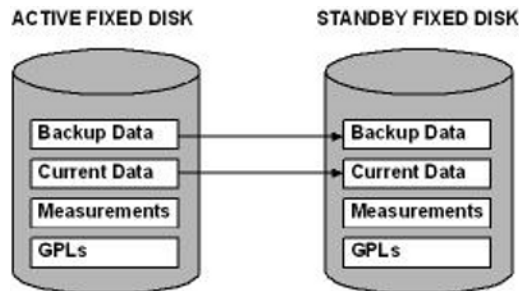
Figure 4-5 chg-db:action=repair
