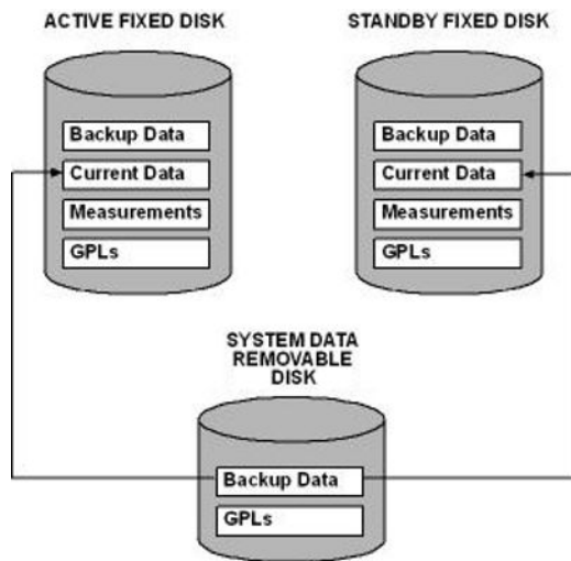
Figure 4-6 chg-db:action=restore:src=remove
