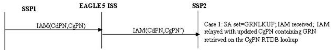
Figure 3-23 ISUP IAM Message Flows for TIF GRN for TIF CgPN Service
