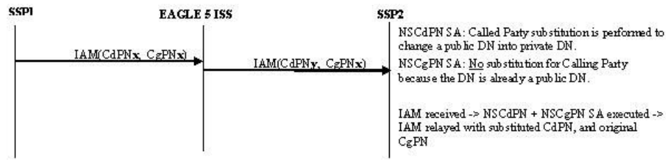
Figure 3-11 ISUP RELAY with TIF NS - No CgPN Substitution
